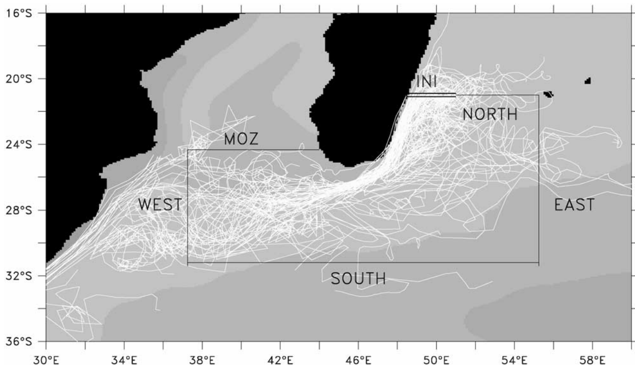
Figure 13. Example float trajectories from the quantitative Lagrangian analysis. Particles were seeded along the double line at 21°S across the SEMC up to 1500m depth, advected by the model velocity and received and summed up at certain control sections (single lines). The control sections (clockwise labeled as NORTH, EAST, SOUTH, WEST, and MOZ) are given in Table 2 (INI is the portion leaving the SEMC northward; DEPTH the portion below 1500 m).
