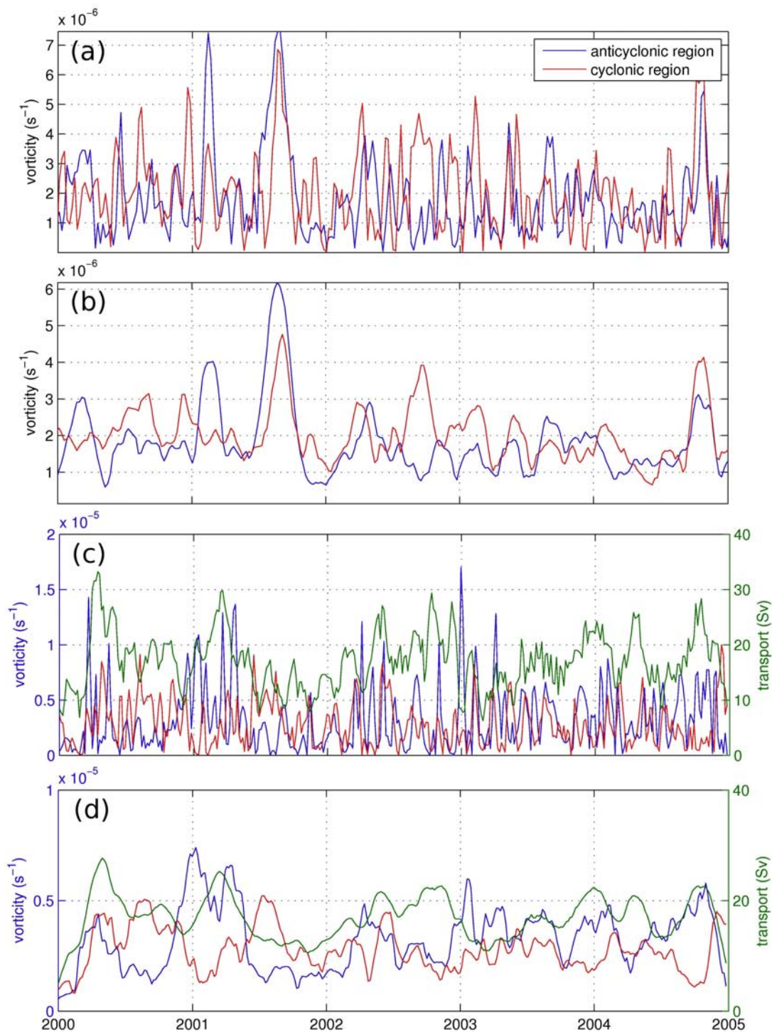
Figure 11. Time series of altimeter vorticity magnitudes (absolute values) in the boxes given in Figure 8: (a) 5-day altimeter data and (b) 2-month moving average of altimeter data. Time series of model vorticity magnitudes in the boxes given in Figure 8 and model transports at 21^{\circ} S (green line): (c) 5-day model data and (d) 2-month moving average of model data.
