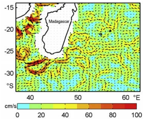
Figure 2. Map of altimeter-derived surface geostrophic currents (6 November 2002, 5-day period) with color indicating speed and the arrows (only every second arrow plotted) presenting velocity.
