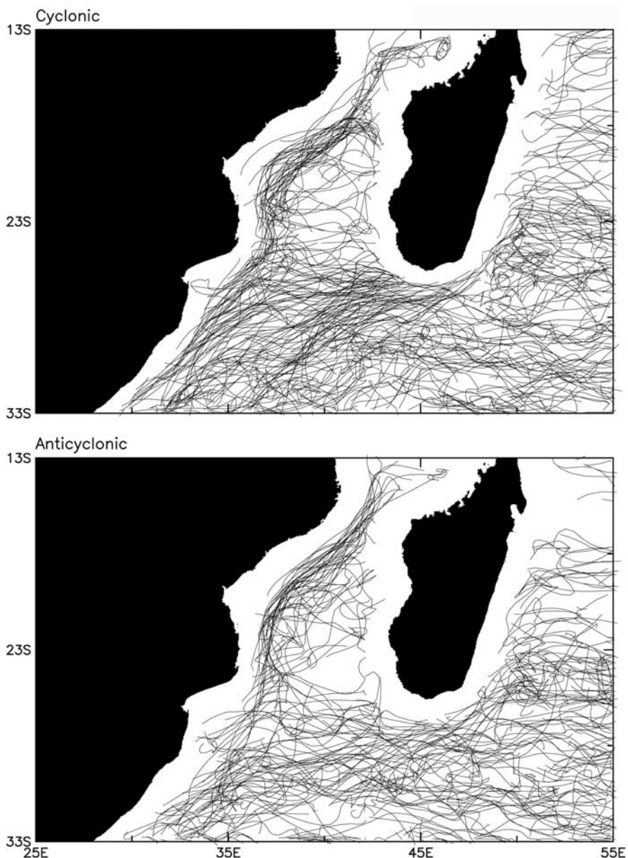
Figure 9. Patterns of (top) cyclonic and (bottom) anticyclonic eddy tracks near Madagascar obtained from altimeter-derived SSH anomalies for eddy lifetimes longer than 16 weeks (courtesy of D. Chelton).
