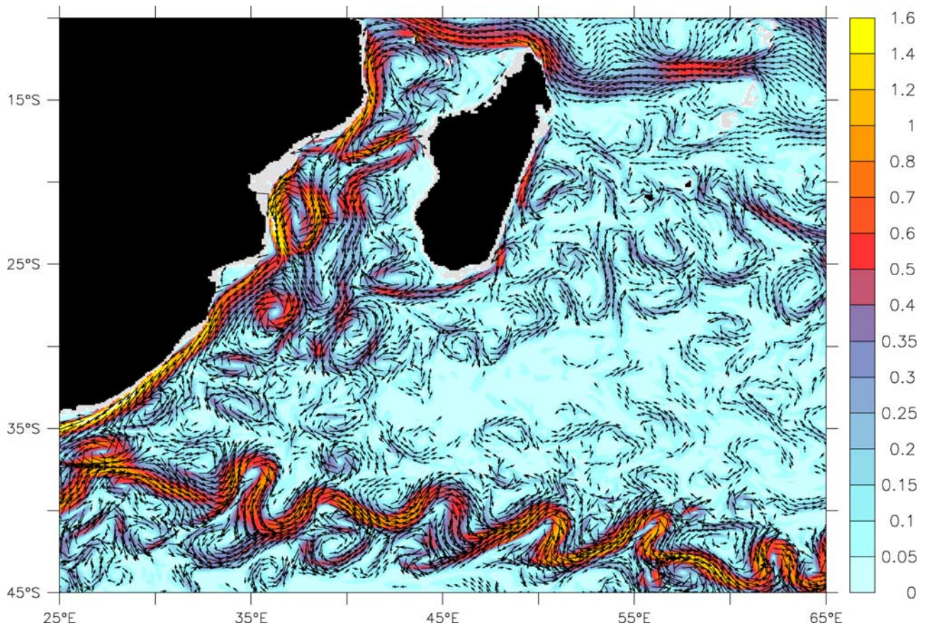
Figure 4. Sample of flow at 100 m from the model, with speed (color bar in m/s) and velocity (every 4th vector shown) as a 5-day average centered around 22 February 1993. Please note the well-represented circulation pattern which is known from observations: the westward South Equatorial Current north of Madagascar, partially leading into southward flow through the Mozambique Channel between Madagascar and the African continent, the Agulhas Current along the South African coastline and the retroflection into the eastward Agulhas Return Current between 35 and 45° S. For a discussion of the flow east and south of Madagascar, please see text.
