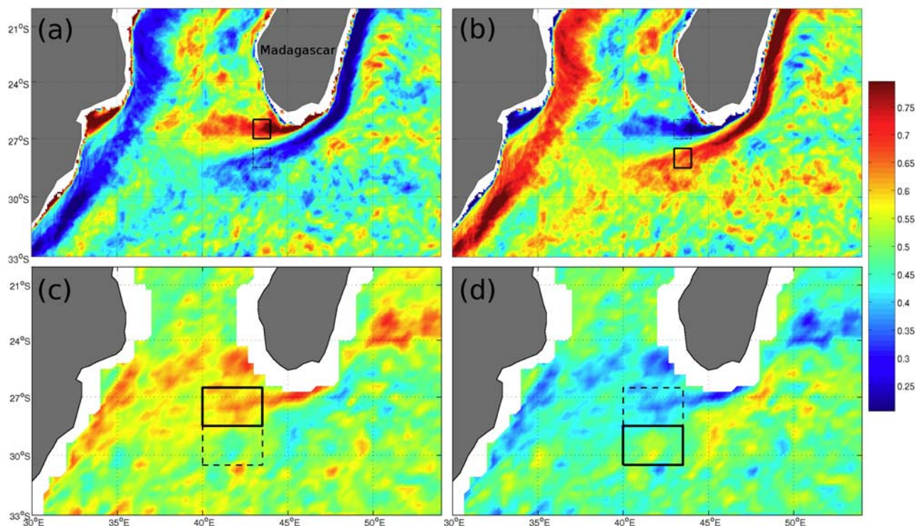
Figure 8. Fractions of (a) cyclonic and (b) anticyclonic EKE from the model and fractions of (c) cyclonic and (d) anticyclonic EKE from altimeter observations relative to the mean EKE, averaged from 1 January 1996 to 31 December 2005. The boxes approximate regions of maximum fractions of EKE in the SEMC extension, with solid-line boxes referring to the particular subfigure and broken-line boxes given for reference.
