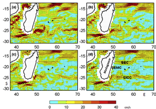
Figure 3. Geostrophic surface currents (only every second arrow plotted) derived from altimeter data averaged over (a) the second half of 2002, (b) the full year 2002, (c) the 2 years 2002–2003, and (d) the 3 years 2002–2004 (SEC is South Equatorial Current; SEMC is southern East Madagascar Current; and SICC is South Indian Ocean Counter-current).
