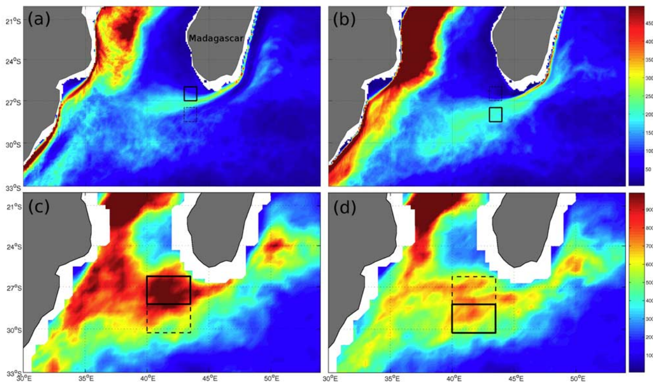
Figure 7. (a) Cyclonic and (b) anticyclonic EKE for currents below the Ekman layer at 100 m from the model and (c) cyclonic and (d) anticyclonic EKE for surface currents from altimeter observations, averaged from 1 January 1996 to 31 December 2005. The boxes refer to Figure 8. Units are \text{cm}^2 \text{s}^{-2} . Please note the different scaling for the upper and lower subfigures.
