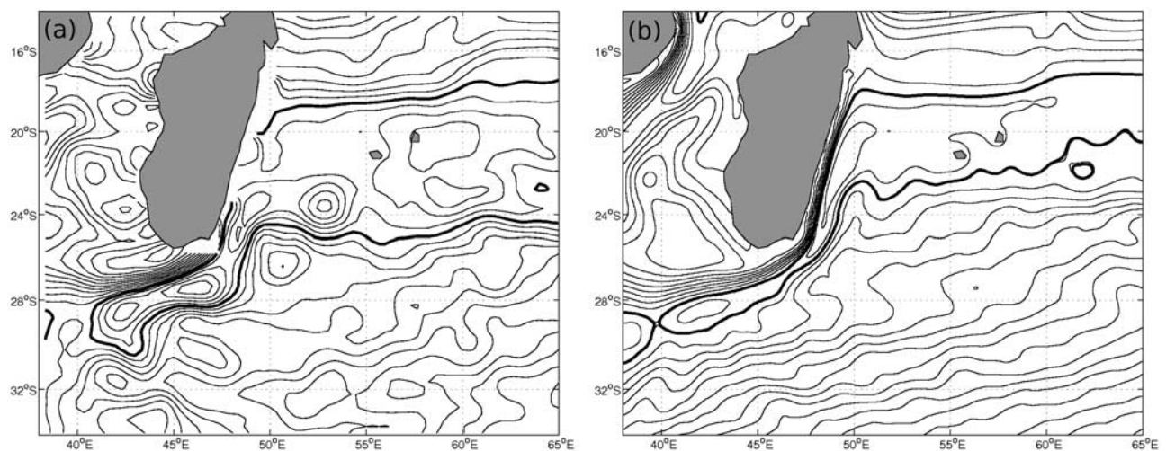
Figure 5. Sea surface height (SSH) maps averaged over 3 years from 1 January 2001 to 31 December 2003, with an isoline interval of 2.5 cm: (a) Aviso altimeter data, (b) model data. The thick lines indicate the 225 cm contour line in Figure 5a and the 220.1 cm contour line in Figure 5b.
