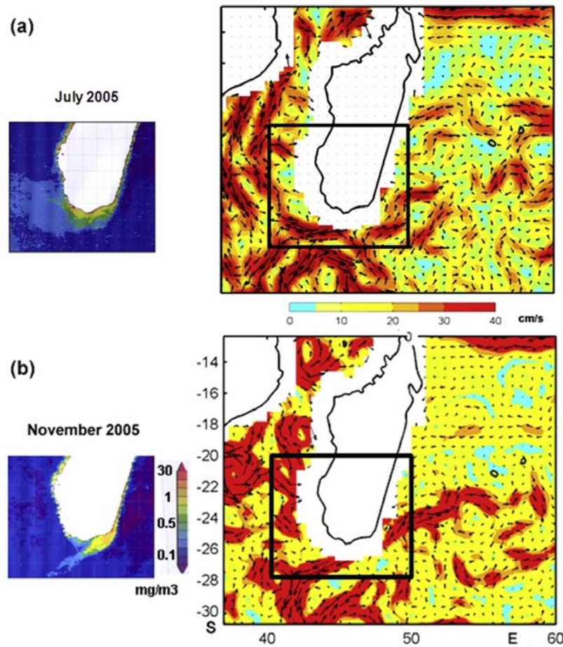
Figure 6. One-month mean distributions for (a) July 2005 and (b) November 2005 showing the modes in SeaWiFS-derived chlorophyll_a patterns and corresponding altimeter-derived geostrophic surface current patterns. The positions of the chlorophyll_a subfigures on the left are indicated in the surface current subfigures on the right.
