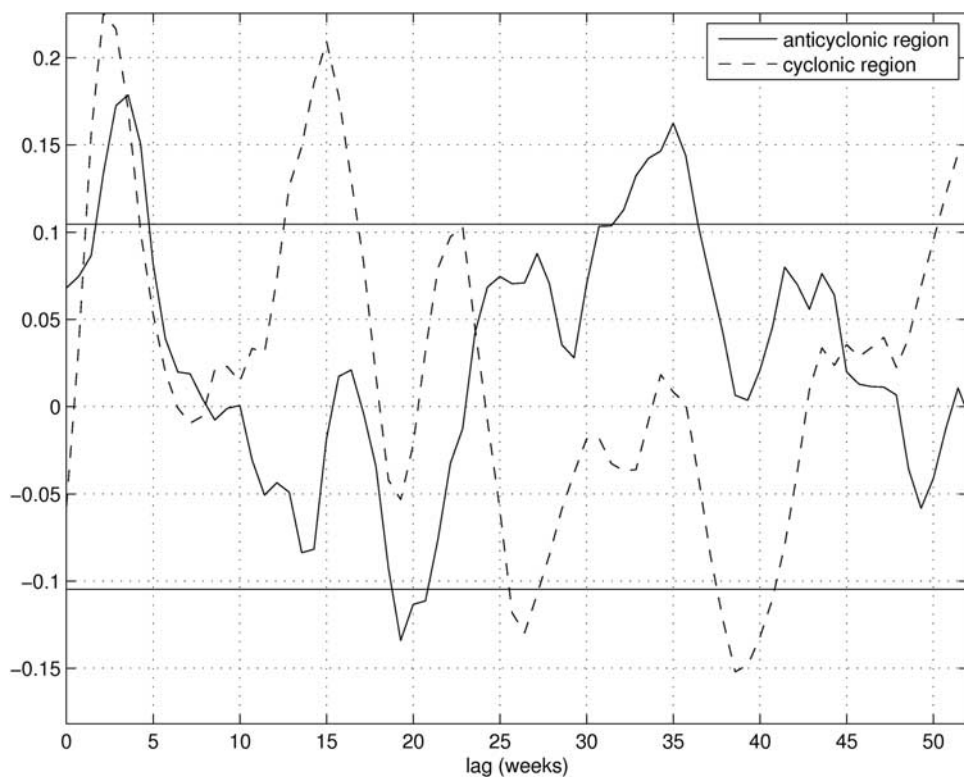
Figure 12. Cross-correlation sequence of SEMC transport at 21° S and cyclonic and anticyclonic motion in the boxes given in Figure 8 from model data. The horizontal lines indicate the 95% confidence level.
