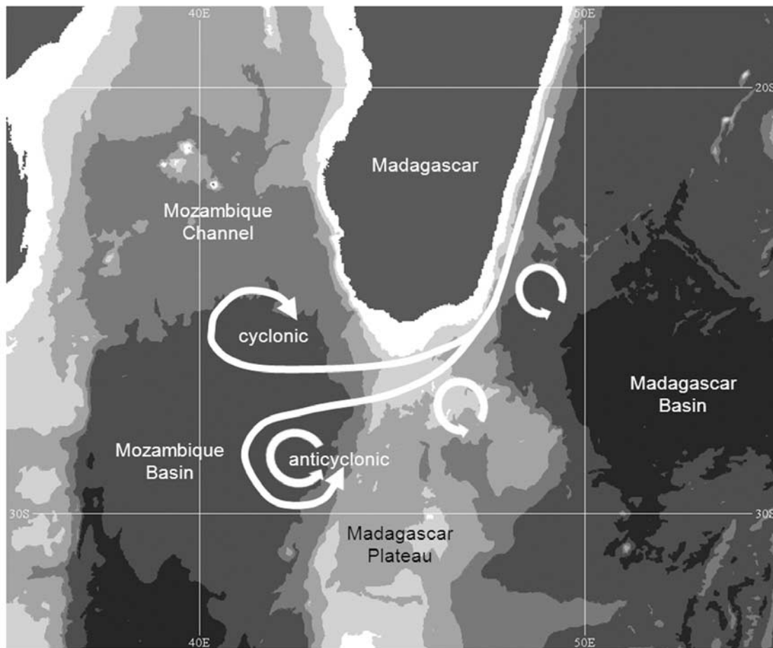
Figure 10. Schematic representation describing the modes of the SEMC extension. The shading indicates isobaths with 1000 m separation where greater depths correspond to darker shading.
