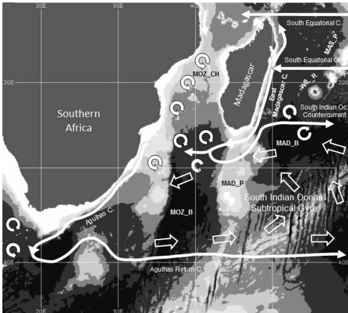
Figure 1. Schematic surface currents (thin solid arrows) in the southwestern Indian Ocean (MOZ_CH is the Mozambique Channel, MOZ_B is the Mozambique Basin, MAD_P is the Madagascar Plateau, MAD_B is the Madagascar Basin, WIL_R is the Wilshaw Ridge, and MAS_P is the Mascarene Plateau). The shading indicates isobaths with 1000 m separation where greater depths correspond to darker shading. The thick open arrows give a simplified pattern of the subtropical gyre following Stramma and Lutjeharms [1997].
