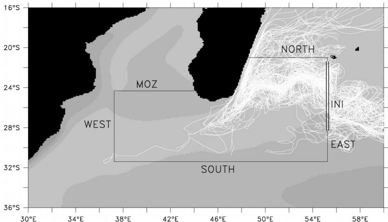
Figure 14. As Figure 13, but floats seeded at 55°E over the SICC and backward calculated. The transports over the control sections are given in Table 3.
