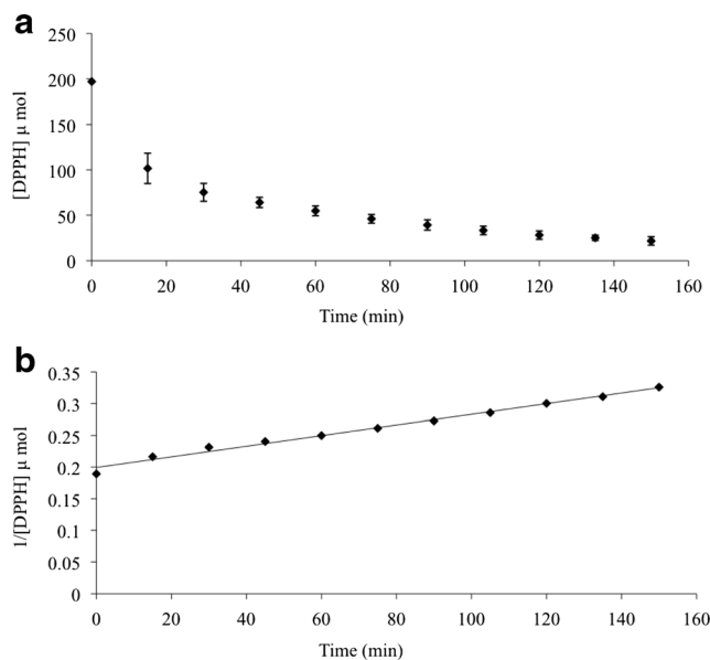
Fig. 2 a DPPH consumed by quercetin-chitosan film versus time. Each data point is an average of five determinations and the error bars show the standard deviation. b 1/\text{DPPH} consumed by quercetin-chitosan film versus time. The black line represents the fitting of the experimental data to the second-order model
