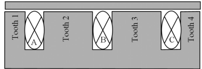
Fig. 3. Axial cross section of a three-phase combined-phase modulated pole machine.
