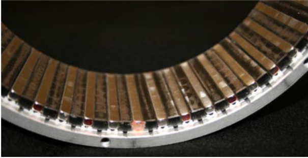
Fig. 14. Close-up view of flux concentrating rotor; the NdFeB magnets are light and the SMC pole pieces are dark.
