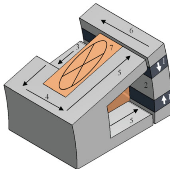
Fig. 1. Two pole section of a single phase.
