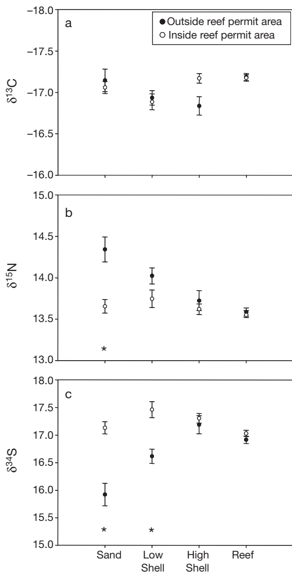
Fig. 6. Lutjanus campechanus . Stable isotope plots of red snapper (a) carbon ( \delta^{13}\text{C} ), (b) nitrogen ( \delta^{15}\text{N} ), and (c) sulfur ( \delta^{34}\text{S} ) collected over sand, low-shell, high-shell, and reef habitats both outside and inside the artificial reef permit area. Asterisks indicate significant differences ( p < 0.05 )
