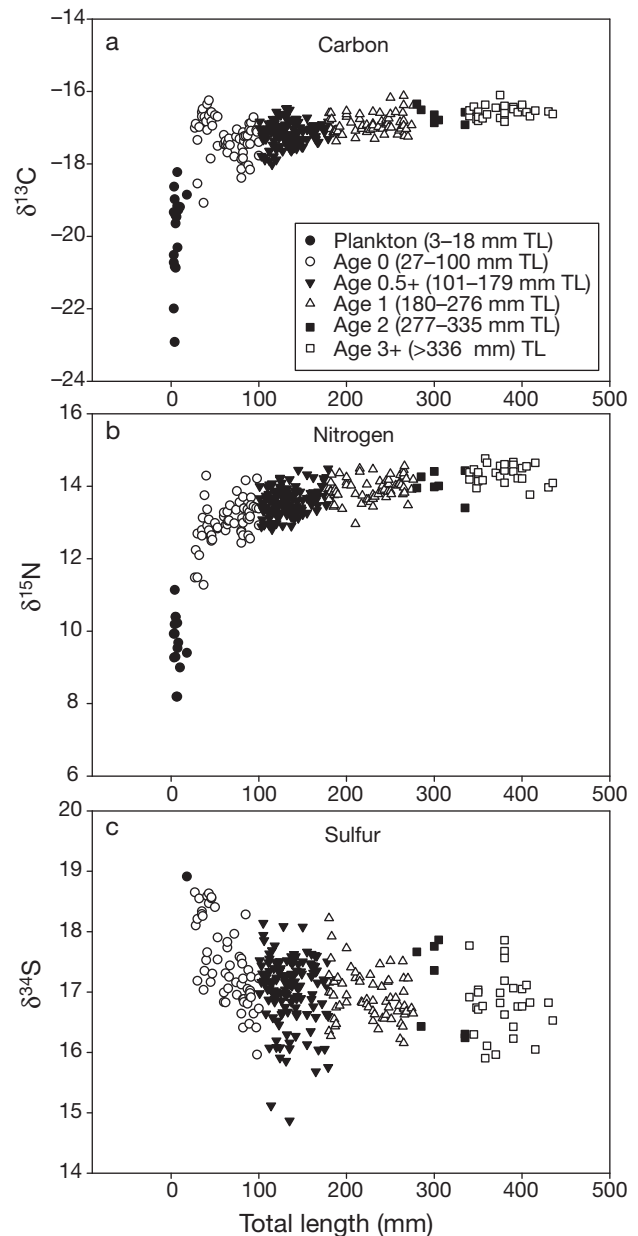
Fig. 3. Lutjanus campechanus . (a) Carbon ( \delta^{13}\text{C} ), (b) nitrogen ( \delta^{15}\text{N} ), and (c) sulfur ( \delta^{34}\text{S} ) as a function of red snapper total length (TL). Specific age groups of red snapper are shown based upon a von Bertalanffy size-at-age model
