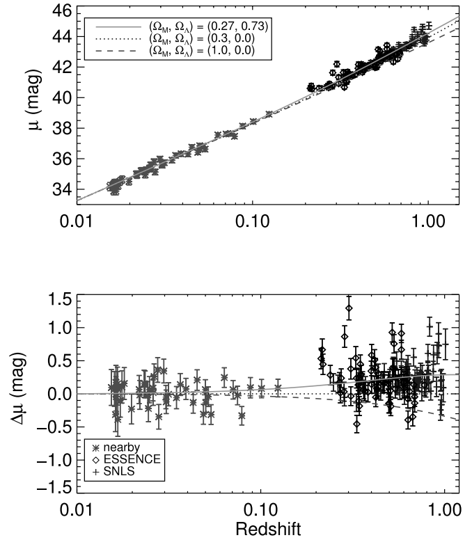
FIG. 9.—Relative luminosity distance modulus vs. redshift for the ESSENCE, SNLS, and nearby SNe Ia for SALT. For comparison, the overplotted solid line and residuals are for a \Lambda CDM ( w, \Omega_M, \Omega_\Lambda ) = (-1, 0.27, 0.73) universe. [See the electronic edition of the Journal for a color version of this figure.]
