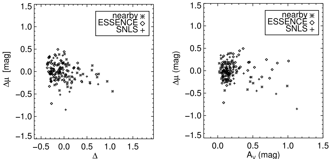
FIG. 3.—Distance modulus ( \mu ) residuals with respect to a \Lambda CDM cosmology as a function of the MLCS2k2 glosz fit parameters: \Delta and A_V . See Table 4. [See the electronic edition of the Journal for a color version of this figure.]
