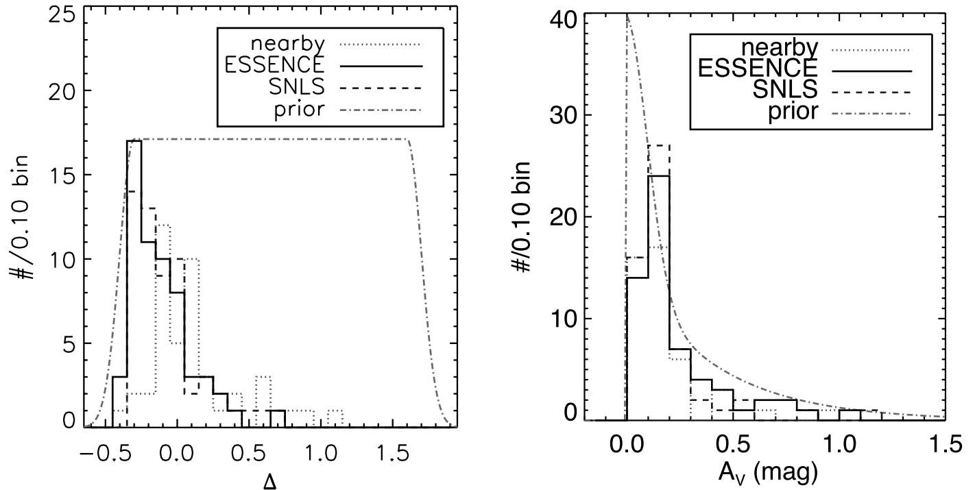
FIG. 1.—Distribution of the MLCS2k2 light-curve width parameter \Delta and A_V for the MLCS2k2 fits with the glosz prior to the nearby (dotted line), ESSENCE (solid line), and SNLS (dashed line) SNe Ia considered in this paper. The glosz prior (dot-dashed line) is shown here for z = 0 , where it is equivalent to the glos prior. Note that we are mixing two slightly different things in showing the prior with these estimated mean fit parameters. The prior, which directly relates to the mode, is not expected to match the a posteriori mean distribution of the fit parameters. See Fig. 7 for the ESSENCE selection effect as a function of redshift. See Table 4 for the full set of MLCS2k2 light-curve fit results for these SNe Ia. [See the electronic edition of the Journal for a color version of this figure.]
