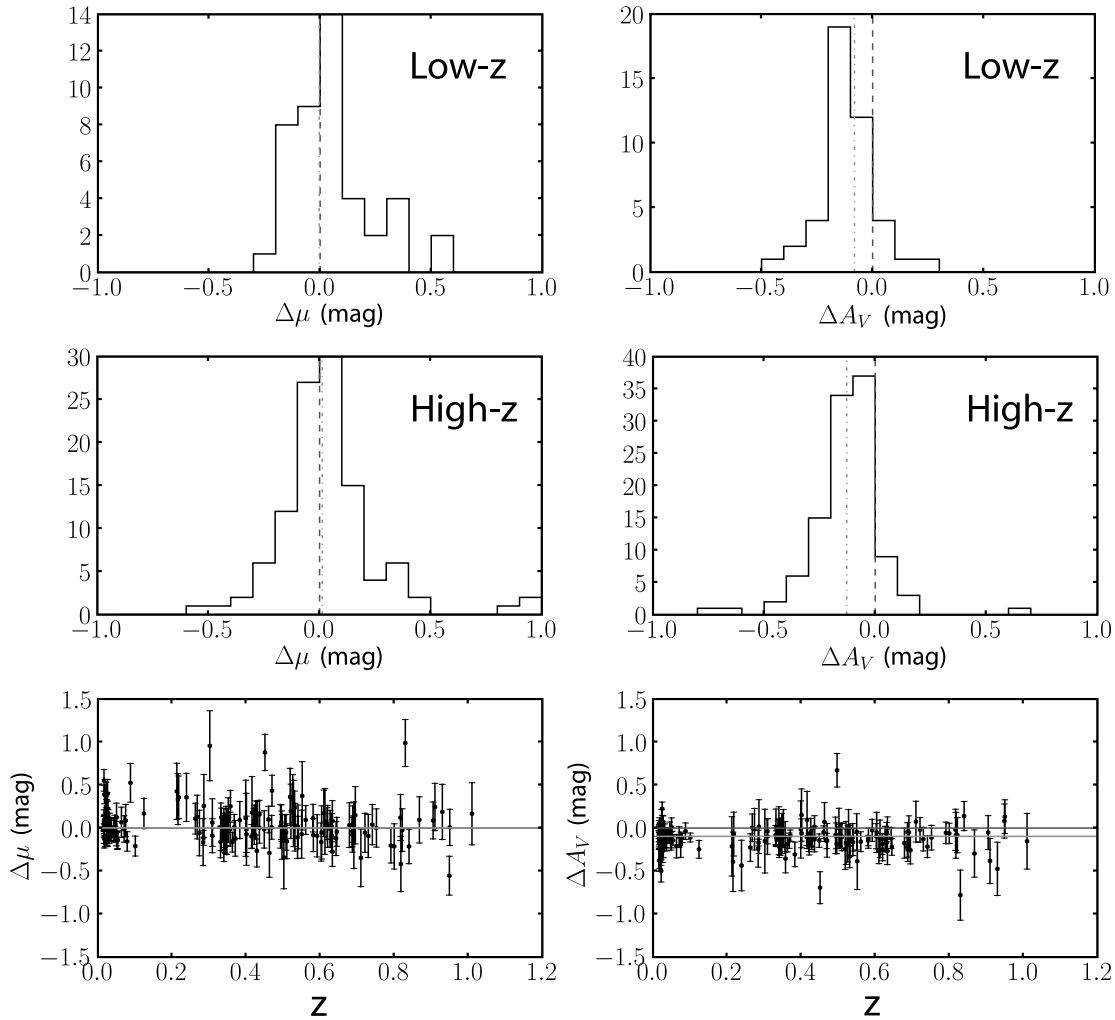
FIG. 5.—Distance modulus and A_V as a function of redshift for MLCS2k2 glosz minus the SALT distance modulus and \beta \times \text{color} ( \beta = 1.57 ) for the ESSENCE, SNLS, and nearby data sets. High z refers to SNe Ia with z \geq 0.15 , low z to z < 0.15 . The dot-dashed line shows the weighted average of the difference for each quantity, while the dashed line shows the line of zero difference. While the luminosity distances are offset between the two fitters, this is mainly due to a slightly different definition of the M parameter that defines the absolute luminosity of an SN Ia and the Hubble constant. The relative average difference between low redshift and high redshift is -0.0023 mag. This agreement translates to a similar agreement in the cosmological parameters obtained with each approach (see Figs. 10 and 11). [See the electronic edition of the Journal for a color version of this figure.]
