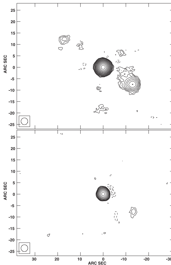
Fig. 2. Combined VLA map of 11 epochs (A, B, C and D-array) of III Zw 2 at 8.4 GHz ( top ) and 15 GHz ( bottom ). All maps were convolved with a beam of 2 \times 2 arcsec to detect faint extended emission. The contours start at 0.12 mJy at 8.4 GHz and 0.6 mJy at 15 GHz, and increase with a factor of \sqrt{2} .
