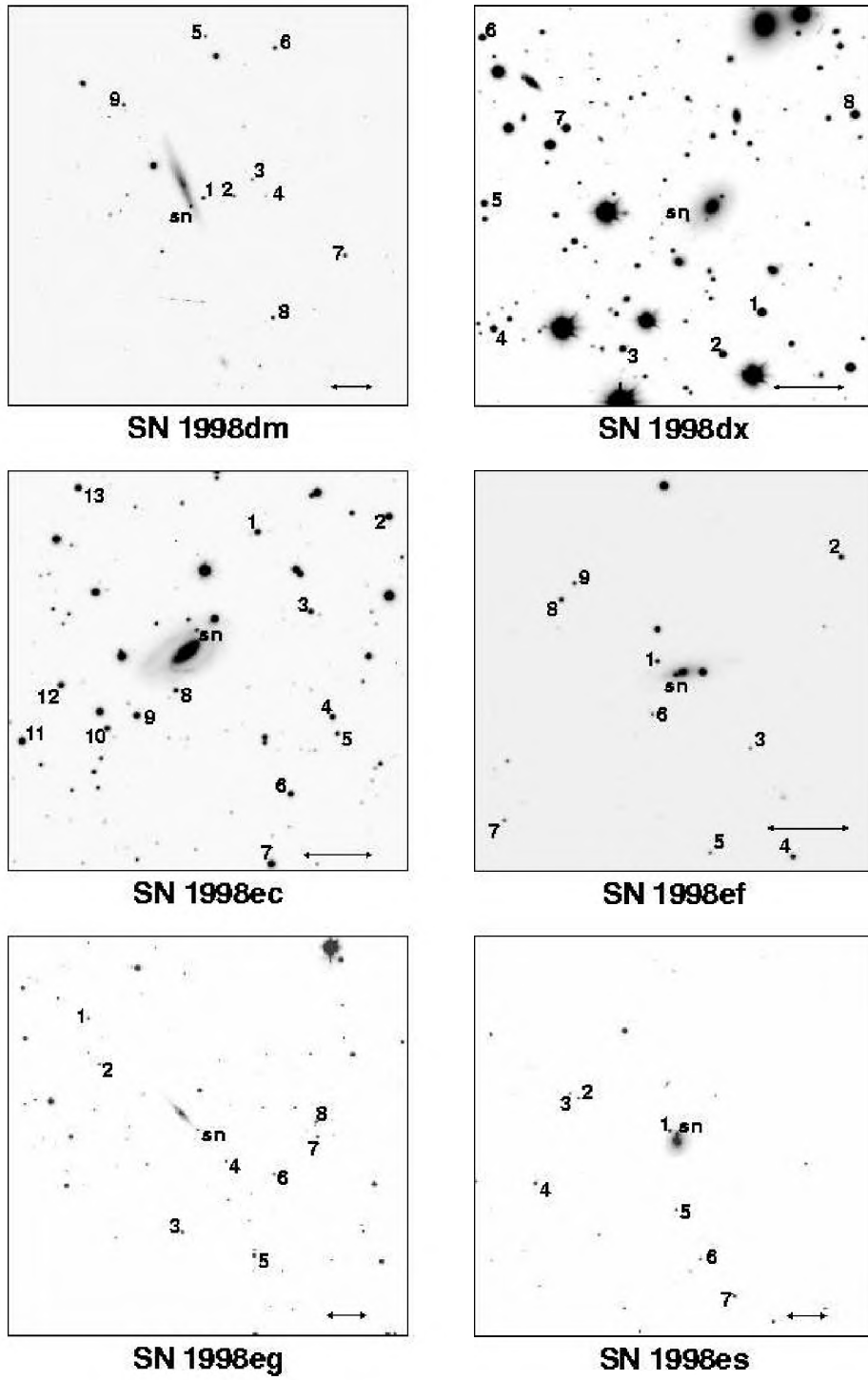
Fig. 1.— Continued
