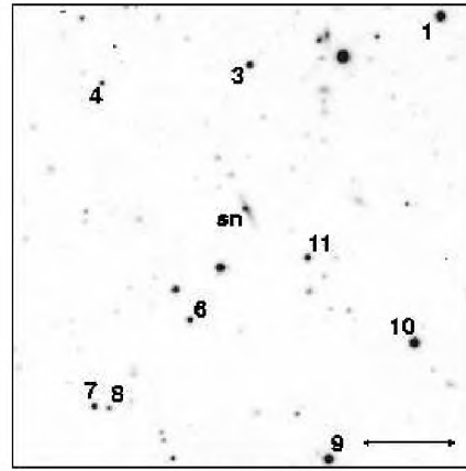
SN 1997dg
