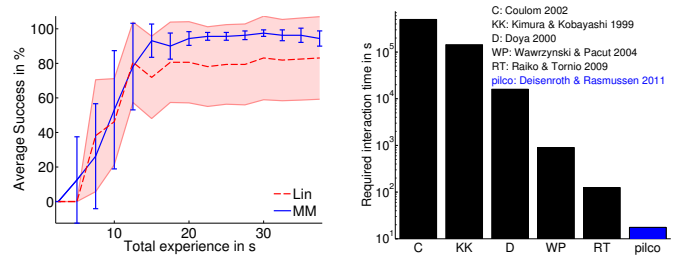
(a) Average learning curves with 95% standard errors: moment matching (MM) and posterior GP linearization (Lin). (b) Required interaction time of different RL algorithms for learning the cart-pole swing-up from scratch, shown on a log scale.
