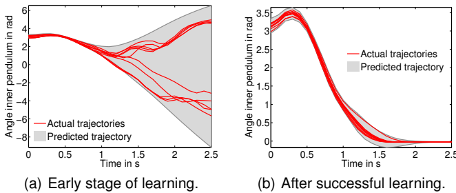
Fig. 9. Long-term predictive (Gaussian) distributions during planning (shaded) and sample rollouts (red). (a) In the early stages of learning, the Gaussian approximation is a suboptimal choice. (b) PILCO learned a controller such that the Gaussian approximations of the predictive states are good. Note the different scales in (a) and (b).
