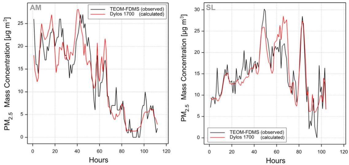
Fig. 4. Comparison of hourly-average PM_{2.5} mass concentrations calculated from the Dylos' linear correlation function with TEOM-FDMS measured PM_{2.5} mass concentrations in \mu\text{g}/\text{m}^3 for Auchencorth Moss ( Outdoor rural , left) and Edinburgh St. Leonards ( Outdoor urban , right).
