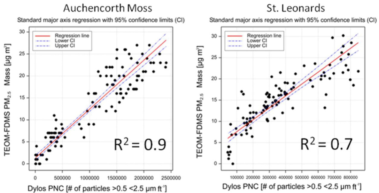
Fig. 3. Comparison of hourly-average PNCs (PNC, # ft -3 for particles between 0.5 and 2.5 μm) from the Dylos monitor and PM 2.5 particle mass (in μg/m 3 ) from the TEOM-FDMS instruments at Auchencorth Moss (left) and Edinburgh St. Leonards (right). The red line represents the equations from Table 1 used for conversion.
