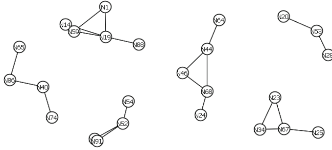
Figure 6: Routers selection using 1-hop egocentric betweenness.
