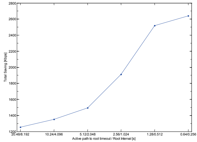
Figure 38: Global bit-rate savings as a function of proactive path lifetimes.
