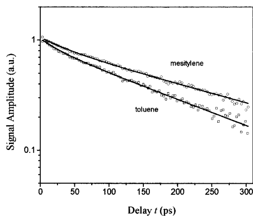
Figure 4. SWM signal amplitudes from the DEANS solutions in mesitylene (○) and toluene (□) as functions of the delay time. Data recorded with all vertical polarizations. The decay is clearly slower in the more viscous solvent. The solid curves are the dynamics predicted by the orientational relaxation model with \Theta = 2.0 \times 10^{-3} \text{ ps}^{-1} and \Theta = 2.70 \times 10^{-3} \text{ ps}^{-1} for mesitylene and toluene, respectively. Note that the time zero signal is not resolved in these lower time-resolution measurements.
