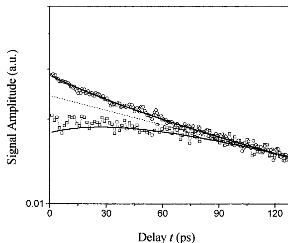
Figure 3. The time-dependence of the signal amplitudes with the two different polarization arrangements for a DEANS solution in mesitylene: (○) are the measured data for all vertical polarizations and (□) for vertical beams 1 and 2, beam 3 at 45°, and detection of the horizontal component of beam 4. The different dynamics are well fitted by (12) and (13) (solid lines) with the assumption of a single rotational diffusion coefficient, \Theta = 2.0 \times 10^{-3} \text{ ps}^{-1} . The dotted line is a single-exponential fit to the data at t > 120 \text{ ps} .
