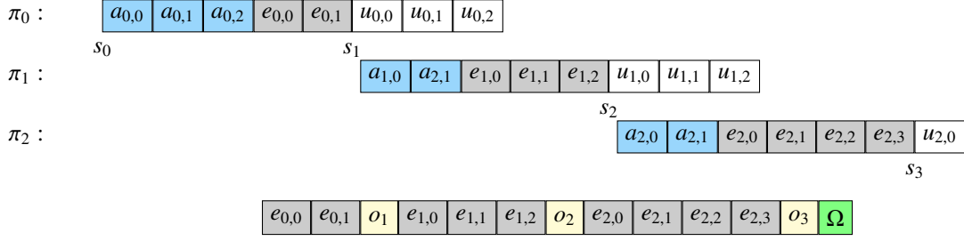
Figure 11: The action sequence (bottom row) enforced on the planner via the action-ordering variable M , so as to reproduce the executed portions of three, partially executed, plans (top three rows). Each observation action o_i requires that the immediately previous physical action resulted in the corresponding observed states s_i .
