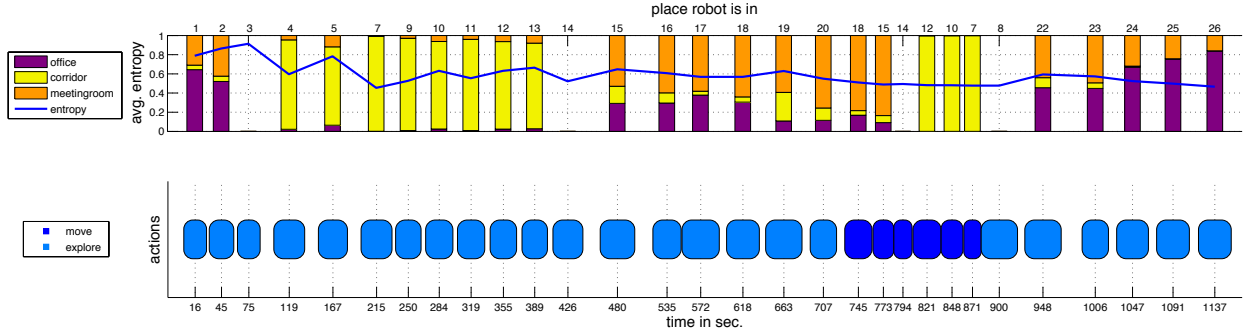
Figure 17: The sequence of the robot’s beliefs (top) and actions (bottom) during an exploration run. The top plot shows the room category distribution after each action. The blue line gives the entropy of the room category distributions, averaged over all rooms found. The numbers at the top refer to the robot’s location, corresponding to the annotations in Figure 16(a). The bottom plot shows the action sequence, indicating execution durations. The action type is colour-coded. Blanks indicate that the robot was planning for that period.
