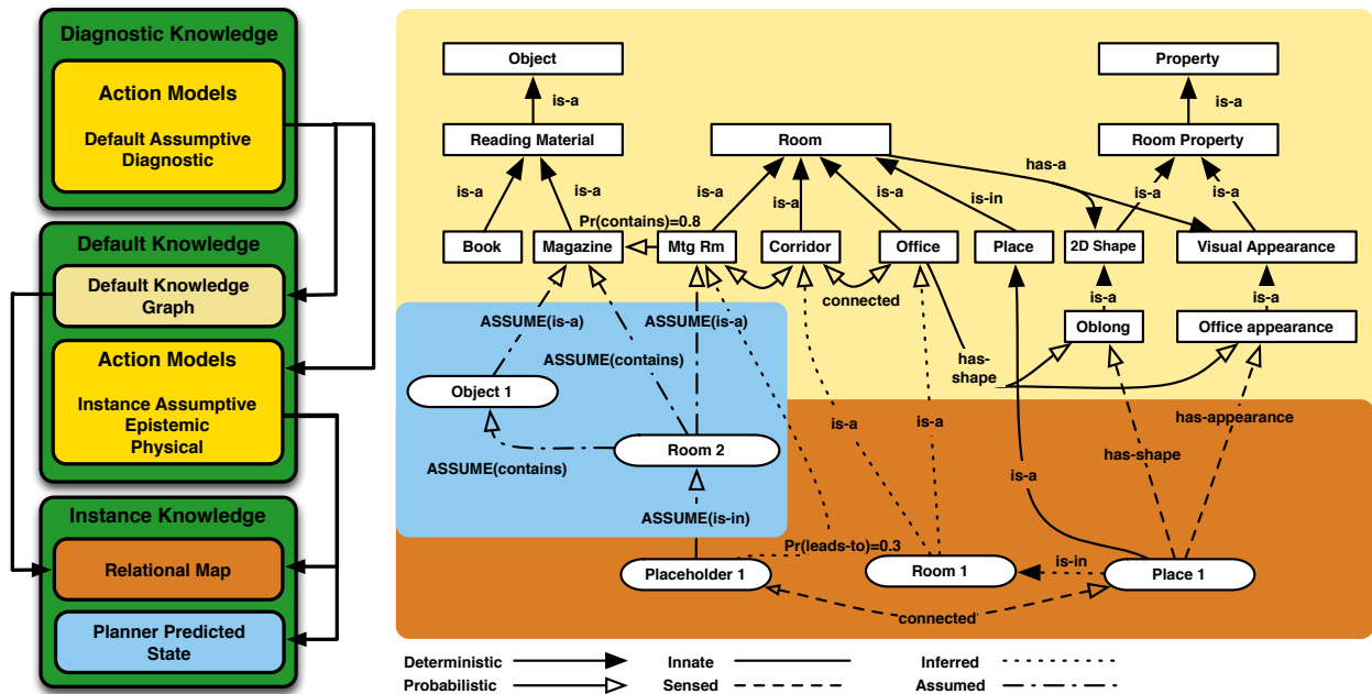
Figure 1: (Left) The instance-default-diagnostic (IDD) knowledge schema, showing action models (yellow), general knowledge (cream), instance knowledge about the current state (brown), and predicted state (blue). (Right) Example state information in the concrete instantiation of the IDD schema used in this paper. The blue box represents possible instance knowledge assumed to be true by the planner in order to achieve the robot's goal (find a magazine). The right panel summarizes the robot's belief state at the start of the running example (see Figure 3).
