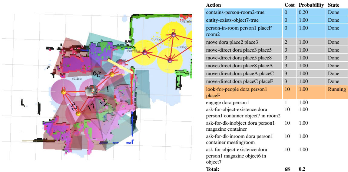
Figure 5: (Left) The robot in the office, at the time of failure. The view cones searched are coloured blue. The robot is in the centre of the room. (Right) The plan to verify the explanation of the failure, showing the three assumptions that need to be made.
