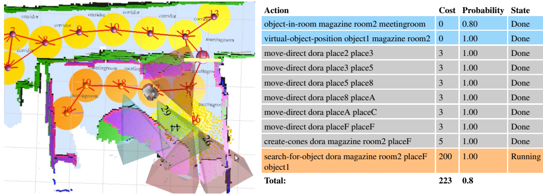
Figure 4: (Left) The map state, three minutes into a run, illustrates the view-planning problem handled by the POMDP planner. The purple tetrahedra are the view cones. (Right) The corresponding plan execution status; grey actions represent completed actions.
