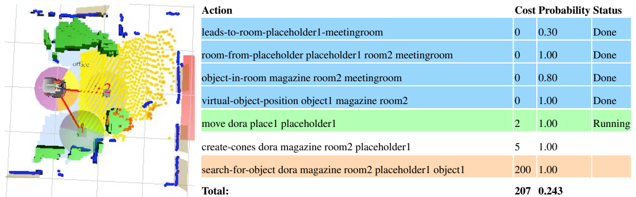
Figure 3: (Left) This shows the initial map state when Dora is switched on. Details are given in the text. (Right) This shows the plan generated for the goal “find a magazine” from the initial state. Light blue entries are assumptive actions, green denotes the current action, white denotes an unexecuted action, and orange denotes a planned call to the decision-theoretic planner. The probabilities of success for each step are taken, by the planner, from the relational map.
