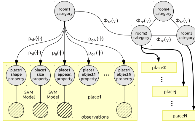
Figure 6: This shows the structure of the chain graph model, compiled from the relational model. The vertices represent random variables. The edges represent the directed and undirected probabilistic relationships between the random variables. The textured vertices indicate observations that correspond to sensed evidence.
