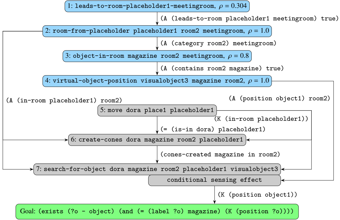
Figure 7: A visualization of the action dependencies of the plan from Figure 3. Assumptions are coloured blue, and physical actions are coloured grey. Arrows indicate that the first action has an effect which the second action depends on via preconditions or conditional effects.
