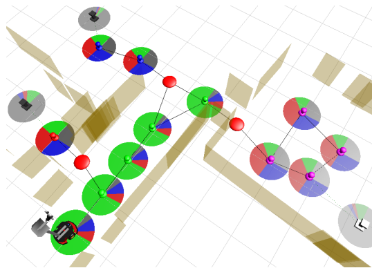
Figure 13: A place map with several places and three detected doors shown as red dots. Colours on circular discs indicate the probability of room categories as in a pie chart. Here green is corridor , red is kitchen and blue is office . Grey circles denote place-holders in unexplored space.
