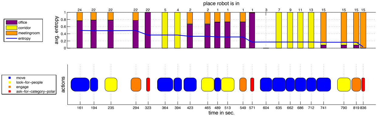
Figure 18: Course of action and the robot’s belief about the categories of rooms in an example categorization run, initiated at the end of the exploration run in Figure 17 that resulted in the map in Figure 16(a). Note the monotonic decrease in the robot’s uncertainty.
