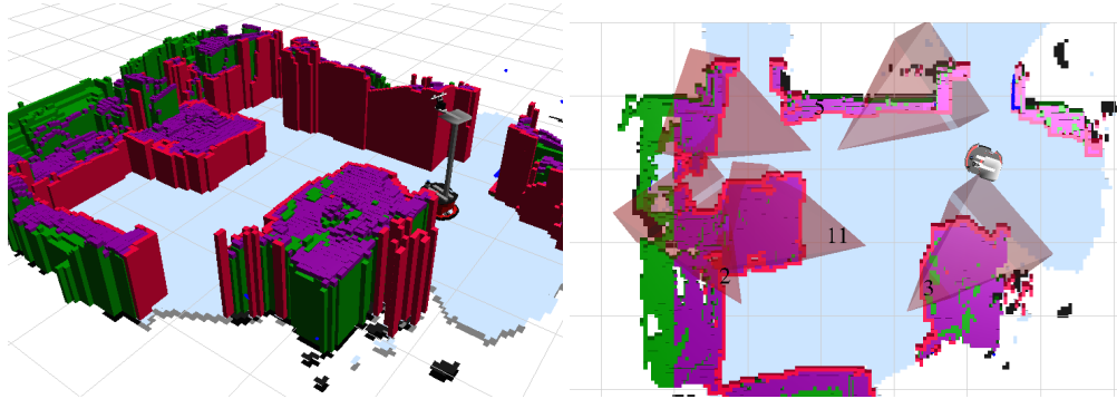
Figure 14: Creating view-point actions for object search. (Left) The prior probability distribution for an object in a room (purple), based on the locations of likely supporting surfaces (green). (Right) Examples of view cones with probabilities.
