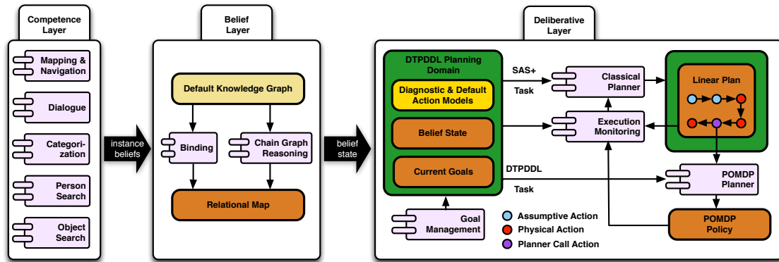
Figure 2: The overall architecture shows how the belief-state maintenance and the switching planner are structured and linked to the basic competences for sensing and action. The implementation of this architecture is described in Section 6.
