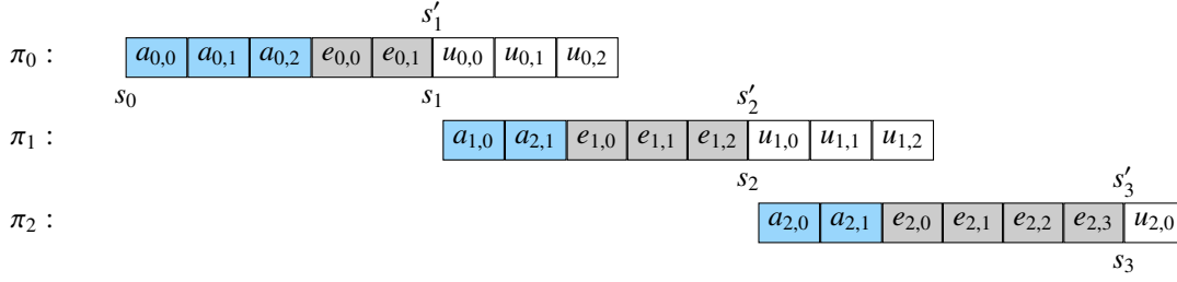
Figure 9: A continual planning process consisting of three planning cycles. Assumptions are coloured in blue, and executed actions are coloured in grey. The state resulting from execution of the last action in a plan (e.g. e_{0,1} ) is the initial state for the next planning cycle.
