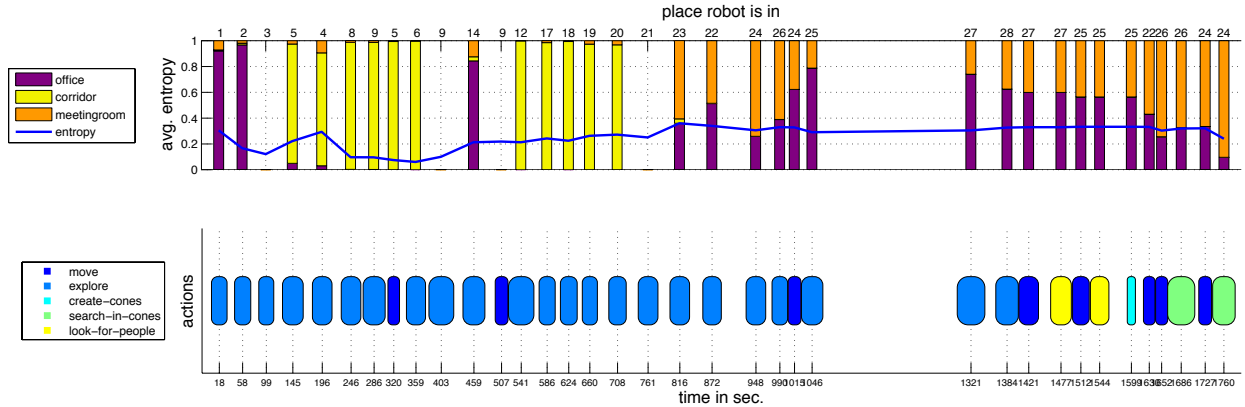
Figure 20: Course of actions in an example object-search run.
