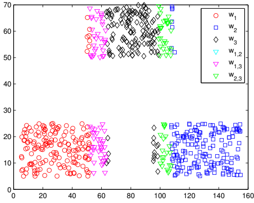
(e). Classification result only by 2 nd step of SCCAI ( Re = 4.83 , Ri_2 = 19.33 , time = 0.1719s ).
