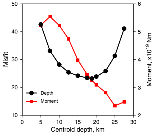
Figure 6. Body wave misfit versus centroid depth. The minimum misfit is at 19 km, but the increase in misfit to the seismograms is less than 15% over the depth interval 15–20 km. The trade-off in moment with depth is shown by the red line.
