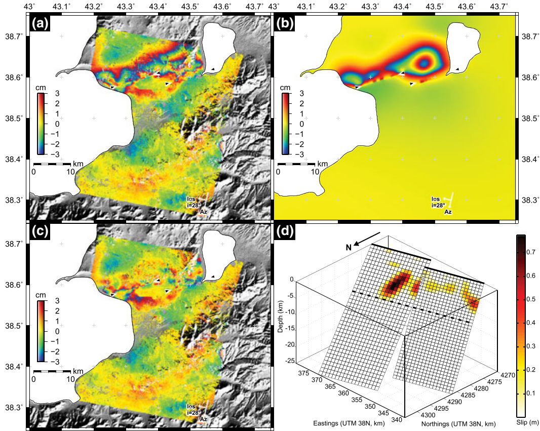
Figure 13. (a) COSMO-SkyMed postseismic interferogram formed from an acquisition 4 h after the earthquake and 3 days afterward. Black and white triangles delineate the two fault segments. A phase discontinuity is visible of the western portion, and a bulls-eye two-fringe lobe is visible just north of the eastern segment. Colors show range changes as fringes re-wrapped to 6 cm, with color cycles blue to red indicating motion away from the satellite for the three satellite tracks. Satellite track azimuth (Az) and line-of-sight (LOS) with angle of incidence ( i ) are shown by white arrows. (b) Model of aftershock/afterslip distribution. (c) Residuals. (d) Afterslip model from the COSMO-SkyMed postseismic interferogram, resolved on the fault planes from the main earthquake. The upper limit of rupture in the main event is delineated by the dashed line.
