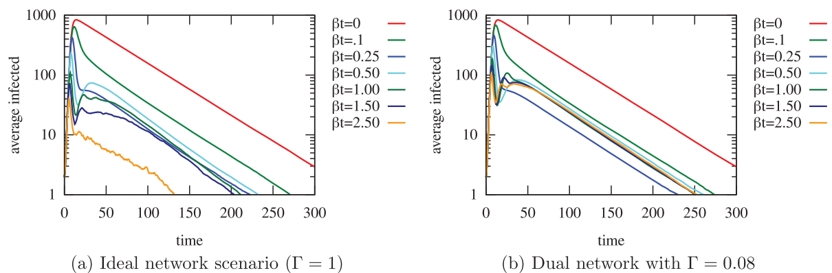
Figure 6. Time varying simulation results of the ideal network scenario and the proposed dual network topology. The infected population plot as a function of time for (a) \Gamma=1 and (b) a network overlap of \Gamma=0.08 , where \alpha=0.1 , \beta_r=0.1 , \gamma=0.5 , K=10 . Contact tracing is always beneficial, even when there is a small overlap between N_i and N_r . We observe that contact tracing becomes increasingly effective as the number of infections increases in both network topologies (a) and (b). However, contact tracing becomes decreasingly effective as the number of infections decreases, particularly in the dual network topology case. This can be seen by the worsened effects of the second and sometimes third peaks for the dual network case (e.g., with \beta_t=2.5 ).
