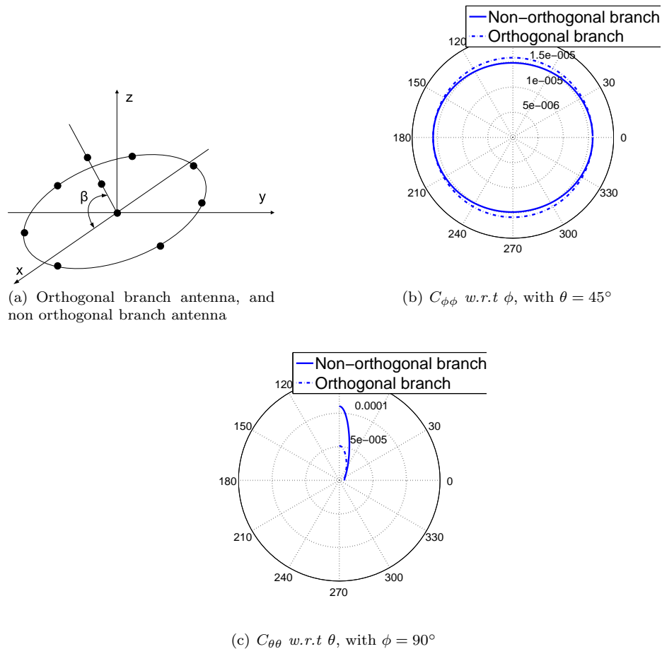
Fig. 2 Orthogonal branch versus non-orthogonal branch antenna.
