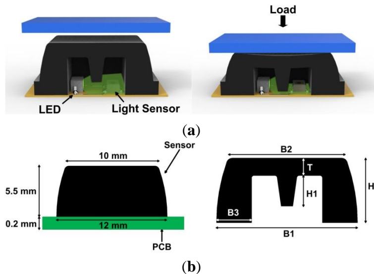
Figure 2. (a) Overview of the sensitive element and its functioning principle; (b) cross-section of the silicone cover; for the pressure-sensitive elements we chose the following values for the constructive parameters: B1 = 12 mm, B2 = 10 mm, B3 = 3 mm, H1 = 2.6 mm, H2 = 5.5 mm, T = 1.5 mm.
