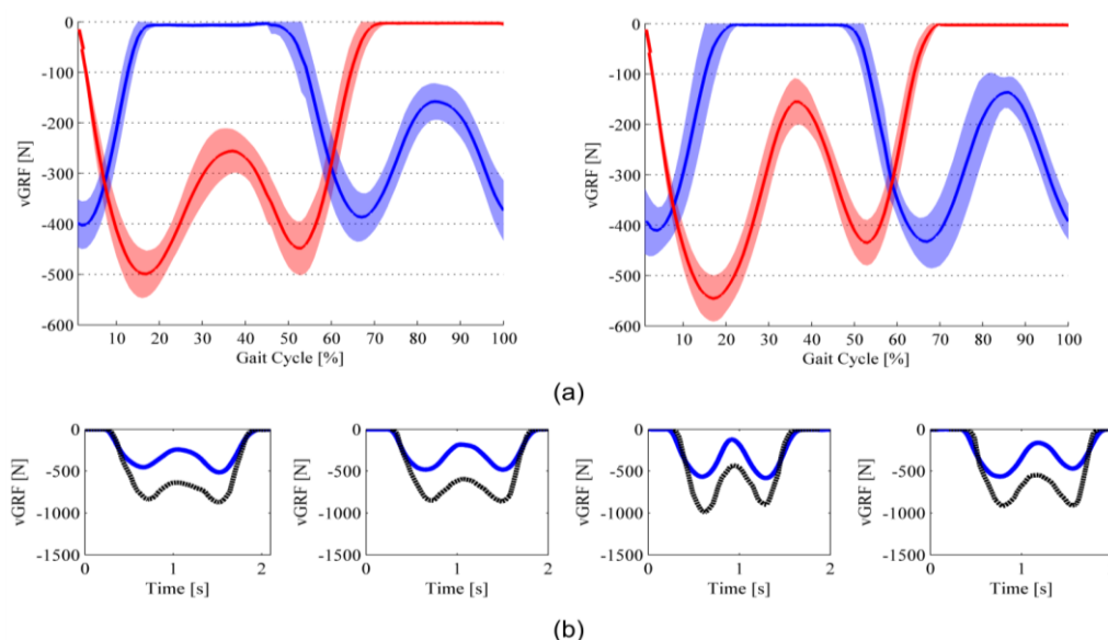
Figure 8. vGRF profiles of Subject #1. Red line is the left foot; blue line is the right foot. (a) Average curve during slow- (on the left panel) and normal- (on the right panel) speed ground-level walking; (b) Comparison between the vGRF profile measured through the sensorized insole (solid blue line) and the force platform (dotted black line) in four different steps.
