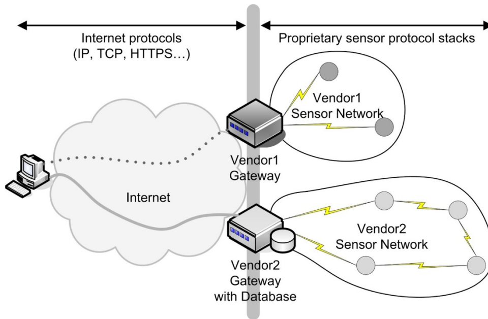
Figure 1. Gateways and proprietary protocols are often used to interconnect sensor networks to the Internet.
