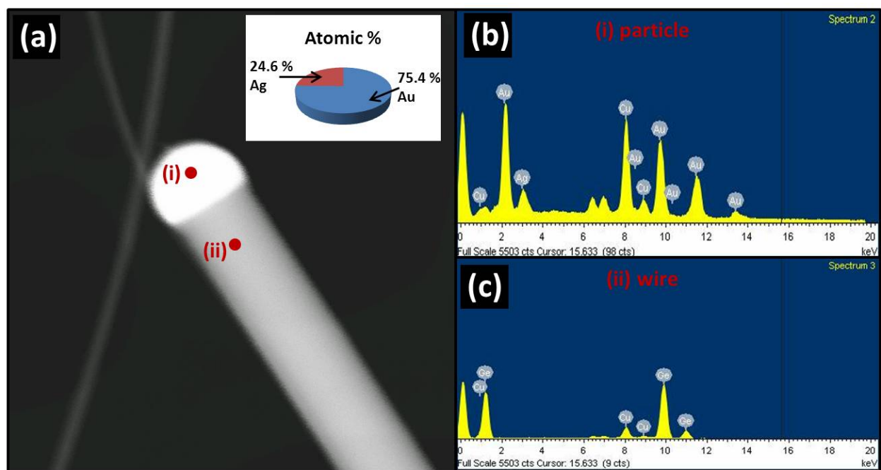
Figure S2. STEM analysis of a Ge nanowire grown from a Au-Ag seed. (a) High angle annular dark field (HAADF) STEM image of a Ge nanowire grown from a Au-Ag seed. Inset shows the atomic % of Ag and Au in the seed particle on top of the nanowire. (b) EDX spectrum of the seed taken at point (i) in (a). (c) EDX spectrum of the wire taken at point (ii) in (a).
