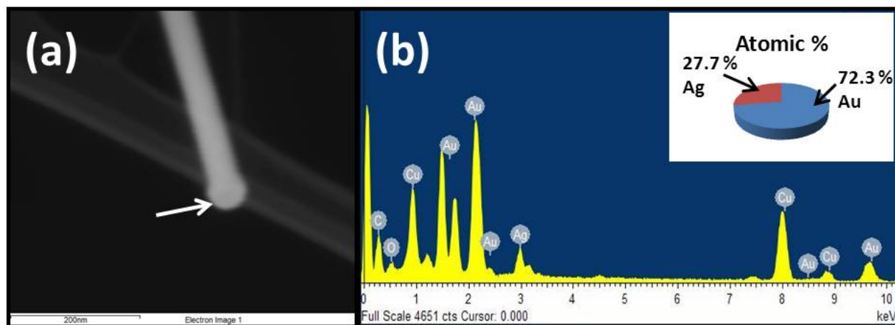
Figure S4. STEM analysis of a Ge nanowire grown from a \text{Au}_{0.75}\text{Ag}_{0.25} nanoparticle. (a) Dark field STEM image of a Ge nanowire grown from a \text{Au}_{0.75}\text{Ag}_{0.25} nanoparticle. (b) EDX spectrum of the seed marked by the white arrow in (a). Inset shows the atomic % of Ag and Au in the seed particle on top of the nanowire.
