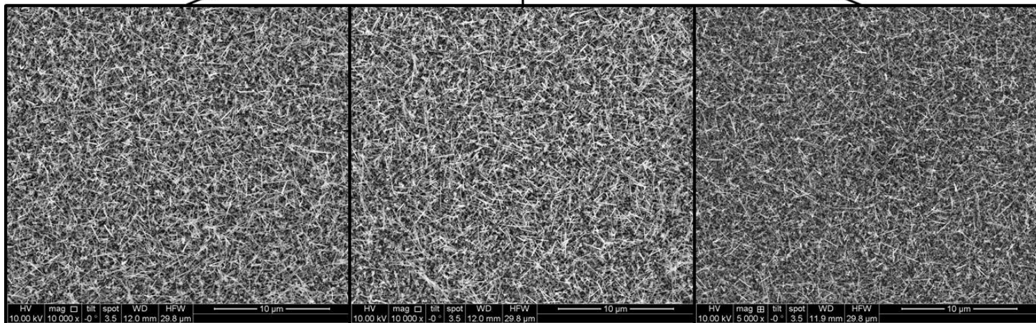
Figure S5. SEM images of Ge nanowires grown from a Au coated substrate. The images show consistent nanowire growth on the left, middle and right portions of the substrate.
