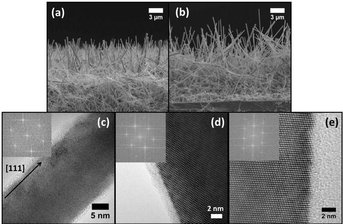
Figure S1. SEM and TEM images showing Ge nanowire growth. (a) SEM image showing Ge nanowires grown from Au-Ge binary alloy catalysts, at a 90 degree angle to the beam (b) SEM image showing Ge nanowires grown from Au-Ag-Ge ternary alloy catalysts at a 90 degree angle to the beam. (c) TEM image of a Ge nanowire grown from a Au film. (d) TEM image of Ge nanowire grown from a Au-Ag bi-layer. (e) Ge nanowire grown from a Au-Ag-Ge tri-layer. The TEM images all show monocrystalline Ge nanowires with a [111] growth orientation. Insets are the fast Fourier transforms (FFTs) taken of the respective nanowires confirming the growth direction.
