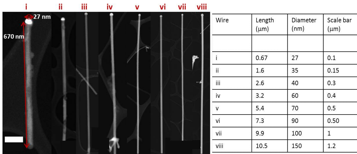
Figure S6. Eight separate STEM images of nanowires synthesised from \text{Au}_{0.75}\text{Ag}_{0.25} nanoparticles. STEM was used to measure the lengths and diameters of nanowires for the Gibbs-Thomson study presented in figure 5(b). The nanowires increase in length and diameter from left to right. Image i shows how the length and diameter were measured and this method was repeated for about 30 nanowires (Au and \text{Au}_{0.75}\text{Ag}_{0.25} seeds), after which the dimensions were plotted in figure 5(b). The table identifies the length and diameter for each nanowire imaged on the left and shows an increasing scale bar from image i to image viii.
