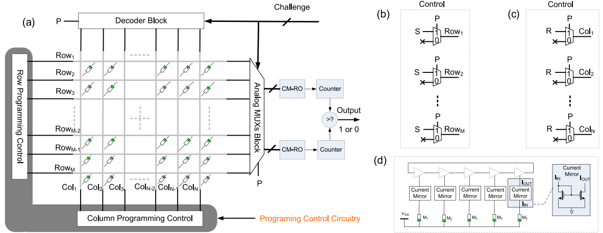
FIGURE 15. mrSPUF architecture. (a) Simplified mrSPUF architecture. All the memristors are in the ON state. The shaded programming control circuit comprises the row programming control circuitry in (b) and column programming control circuitry in (c), which is employed to program memristors in the nanocrossbar array before it acts as a PUF and facilitates reconfigurability of mrSPUF by subsequent reprogramming to refresh CRPs of mrSPUF to transform it into a new PUF instance. In contrast to the programming control circuit, the top decoder block and left analog multiplexers block, CM-ROs and counters enables the stimulation by a challenge and the extraction of a corresponding response. A challenge encoded as a vector of binary values (bits) is used to provide the address bits for both the analog multiplexers block and the decoder block. (d) CM-RO. Each current mirror starves only an inverter in the RO structure, where the bias memristor for each current mirror, M_i , is selected from the nanocrossbar array. Although variation in the oscillation frequency of each CM-RO is slightly influenced by the threshold voltage variation in the CMOS transistor composing the starved inverter and current mirror structures, the overall variation in the oscillation frequency is primarily determined by the variations in memristance of M_i if the supply voltage, V_{DD} , is kept constant.
