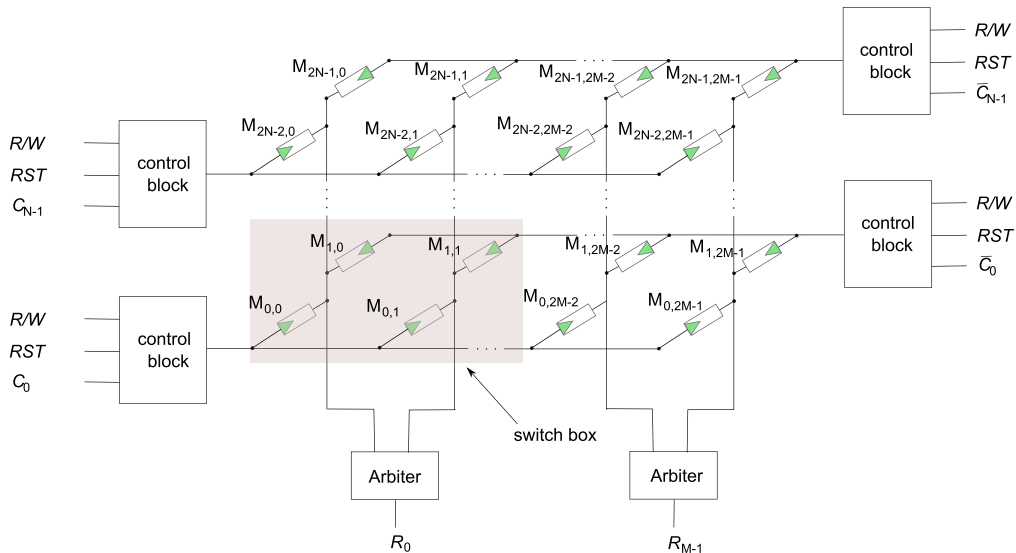
FIGURE 13. Simplified architecture of the XBARPUF for N configuration and M -bit response [27].
