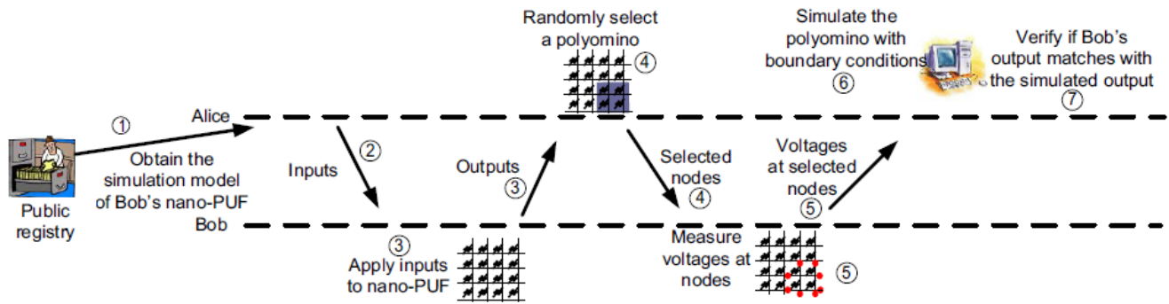
FIGURE 11. Time-bounded authentication protocol using nano PPUF. After [28].
