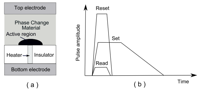
FIGURE 4. (a) A cross-sectional view of a conventional PCM cell. (b) The programming pulse passing through the PCM will change the temperature in the active region using the heater based on the pulse amplitude and duration. The resistance is read out by passing a small amplitude and short duration pulse without disturbing the resistance of the PCM.
