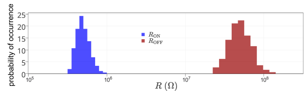
FIGURE 10. Experimental resistance variation distribution extracted from a 40 × 40 nanocrossbar array with 1600 memristors obtained from experimental data in [83].
