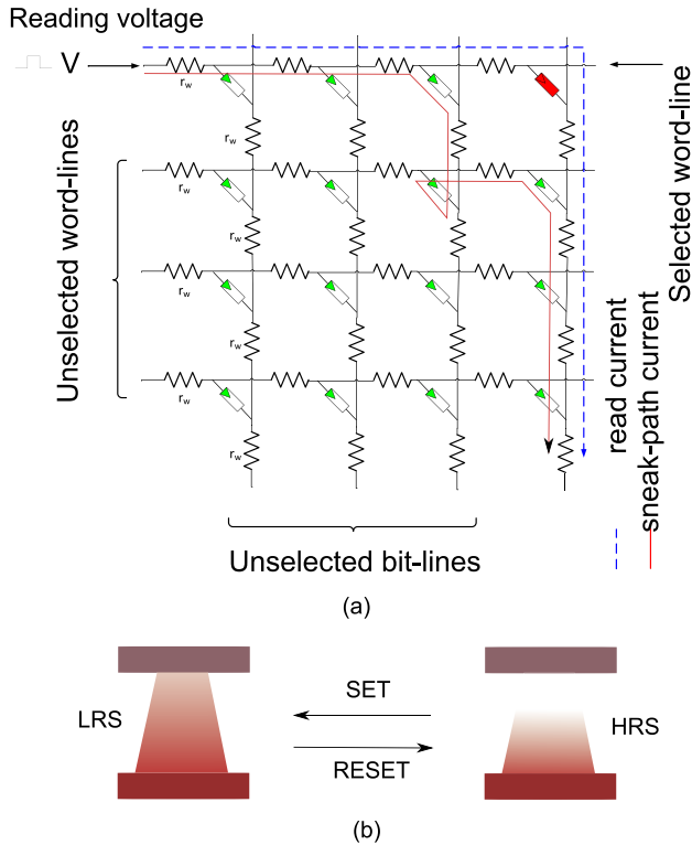
FIGURE 9. Nanocrossbar array and a memristor. (a) Nanocrossbar array of memristors, where each memristor is located at the crosspoint of a top and a bottom electrode. When reading a targeted memristor (selected cell in the top-right corner), reading voltage is targeted applied to the selected word line and the current passing through the selected bit line is sensed to determine the state of the memristor. For other unselected word and bit lines, they can be connected to ground or to a high impedance (floating). During reading it is important to note that there also exists many sneak path currents besides the desired read current. (b) Illustrates the operation principles of a memristor. There is a concentration gradient of filaments that can be moved back and forth using an applied electric field. The memristor switches from a HRS (High Resistance State) to a LRS (Low Resistance State) with a positive potential difference between the bottom electrode and top electrode corresponding to SET switching as one or more conductive filaments grows or forms, while it switches from LRS to HRS with a negative potential difference between the bottom electrode and top electrode corresponding to RESET switching as the filaments are disrupted. Once a memristor has been programmed, its memristance does not change even if its power supply is disconnected unless a voltage higher than a threshold voltage is applied across the device. Note that this is a very simple illustration of the memristor and does not cover all device-physics aspects of switching. After [34].
