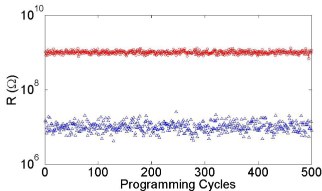
FIGURE 12. Cycle to cycle (C2C) variations. R_{OFF}/HRS and R_{ON}/LRS variation of an individual memristor for 500 cycles, experimental data is adopted from [89].
