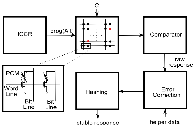
FIGURE 6. Block diagram of PCKGen. The imprecisely controlled current-pulse regulator (ICCR) is responsible for generating imprecise duration and amplitude of the programming pulse to reconfigure the PCM array. Comparator compares resistance of two selected PCM cells (marked with red color)—where the address is determined by a challenge—in the PCM array to generate raw responses.
