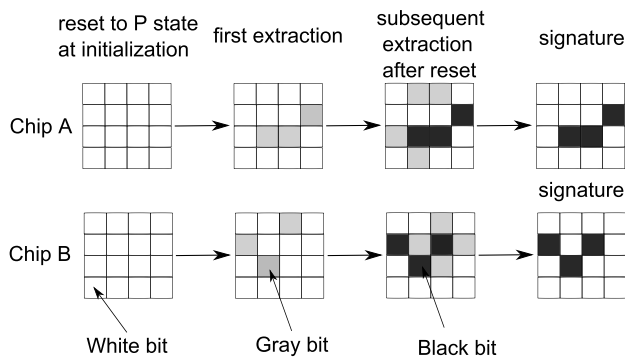
FIGURE 8. Operation sequence for extracting a PUF signature from a 4 × 4 STT-MRAM array. The extracted data is categorized into three patterns: much less than 50% (white), around 50% (gray) and much more than 50% (black). After [20].
