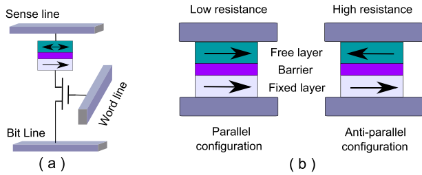
FIGURE 7. (a) The STT-MRAM memory cell. (b) MTJ configuration.
