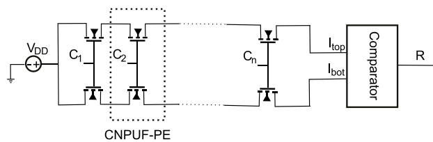
FIGURE 3. CNFET based PUF design (CNPUF).
