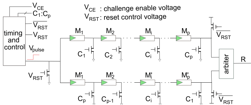
FIGURE 14. Architecture of the proposed memristor-based PUF circuit [32].
