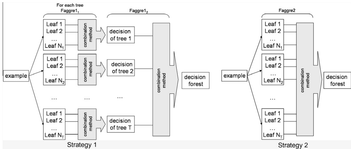
Fig. 1. Strategies for fuzzy classifier module.
