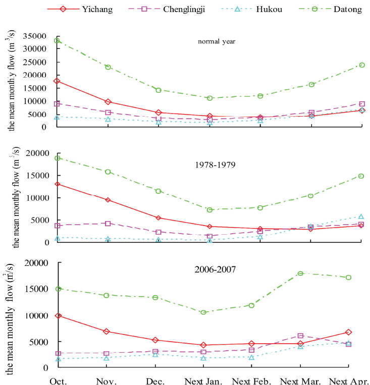
Figure 3 Variations in the mean monthly flow in dry season in different years at Yichagn, Chenglingji, Hukou, Datong hydrological stations
