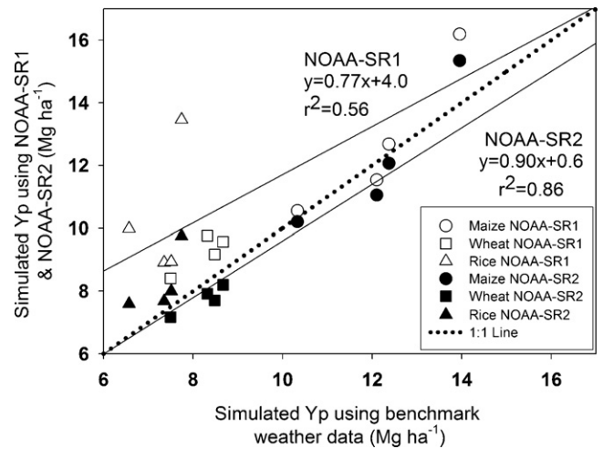
Fig. 2. Comparison of Yp simulated with two sources of NOAA weather data, either using derived solar radiation (NOAA-SR1) or observed solar radiation from the NASA-POWER database (NOAA-SR2) versus a benchmark from weather stations at which all required weather data were directly measured. Values shown represent 19-year means for each of four sites for rice and maize and 10-year means for each of four sites in Germany.
