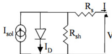
Fig. 1. solar cell equivalent circuit.
