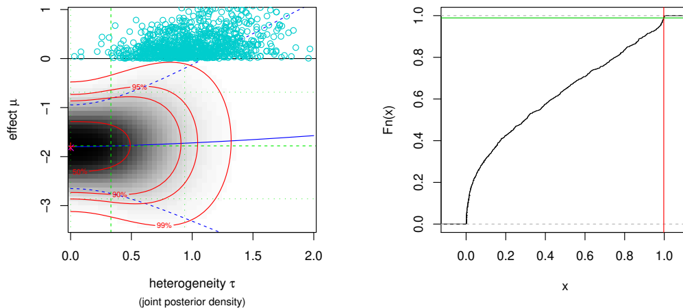
Figure 7: Illustration of the computation of a posterior predictive p value using Monte Carlo sampling. The left panel shows the distribution of replicated \mu^* and \tau^* values, the right panel shows the empirical (cumulative) distribution of the associated “test statistic” values.
