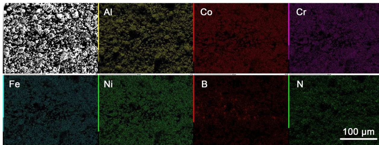
Figure S4 – \text{Al}_2\text{CoCrFeNi} + 3 wt.% h -BN after ball-milling with a Fritsch Planetary Mill PULVERISETTE 5/2 (10 mm steel balls, ball-to-powder ratio 5:1, 5 minutes, 250 r.p.m.).
