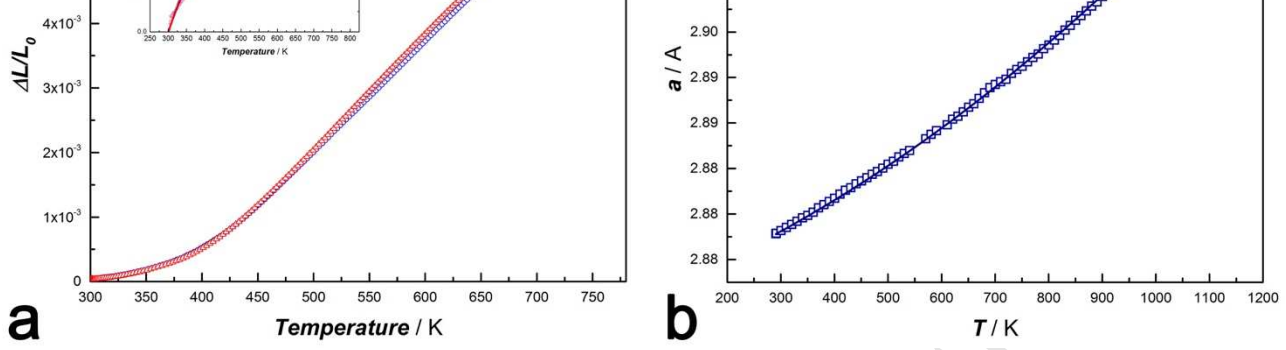
Figure 4 – (a) Thermal expansion of the Al 2 CoCrFeNi HEA (blue) and of its composite material containing 2 wt.% nano-diamonds (red) after spark-plasma sintering. Inset : thermal expansion coefficient from 300 to 770 K, (circles) obtained as CTE_m and (line) obtained as thermal expansivity. (b) Thermal expansion of the cell parameter a from PXR of the as-cast Al 2 CoCrFeNi HEA (DIAMOND Light Source, I11, \lambda=0.494984 Å). Database fitting performed with equation (2).
