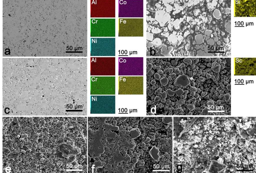
Figure 1- SEM and selected EDX micrographs of (a) \text{Al}_2\text{CoCrFeNi} HEA with element distribution maps; (b) \text{Al}_2\text{CoCrFeNi} + 2wt.% SiC with a distribution map of Si in the sample; (c) \text{Al}_2\text{CoCrFeNi} + 2 wt.% nano-diamonds with element distribution maps of the HEA matrix; (d) \text{Al}_2\text{CoCrFeNi} + 0.5 wt.% \text{Sc}_2\text{O}_3 with a distribution map of Sc in the sample; (e) \text{Al}_2\text{CoCrFeNi} + 3 wt.% h-BN; (f) \text{Al}_2\text{CoCrFeNi} + 2 wt.% c-BN; (g) \text{Al}_2\text{CoCrFeNi} + 1.5 wt.% CN.
