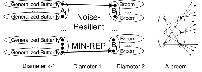
Figure 1: TC-spanner instance \mathcal{G} & an example of a broom.
