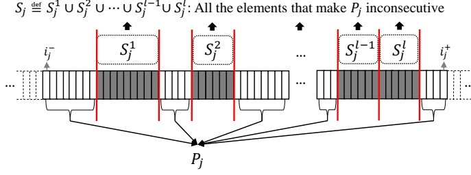
Fig. 3. An illustration of records from one partition P_j lying in a non-consecutive way in the sorted CT.
