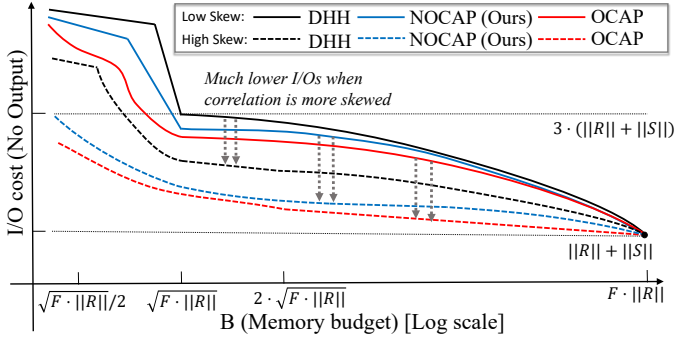
Fig. 1. A conceptual graph on the I/O cost of the state-of-the-art DHH, OCAP and NOCAP, assuming \|R\| \leq \|S\| . F is the fudge factor indicating the space amplification factor between the in-memory hash table and the stored raw data).
