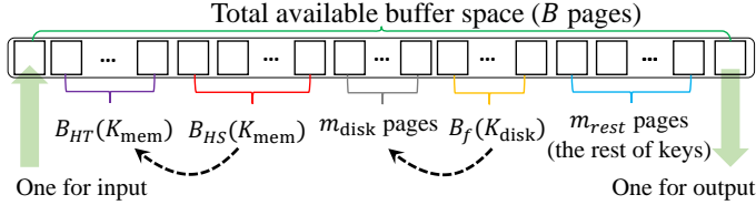
Fig. 6. The memory breakdown when partitioning R .
