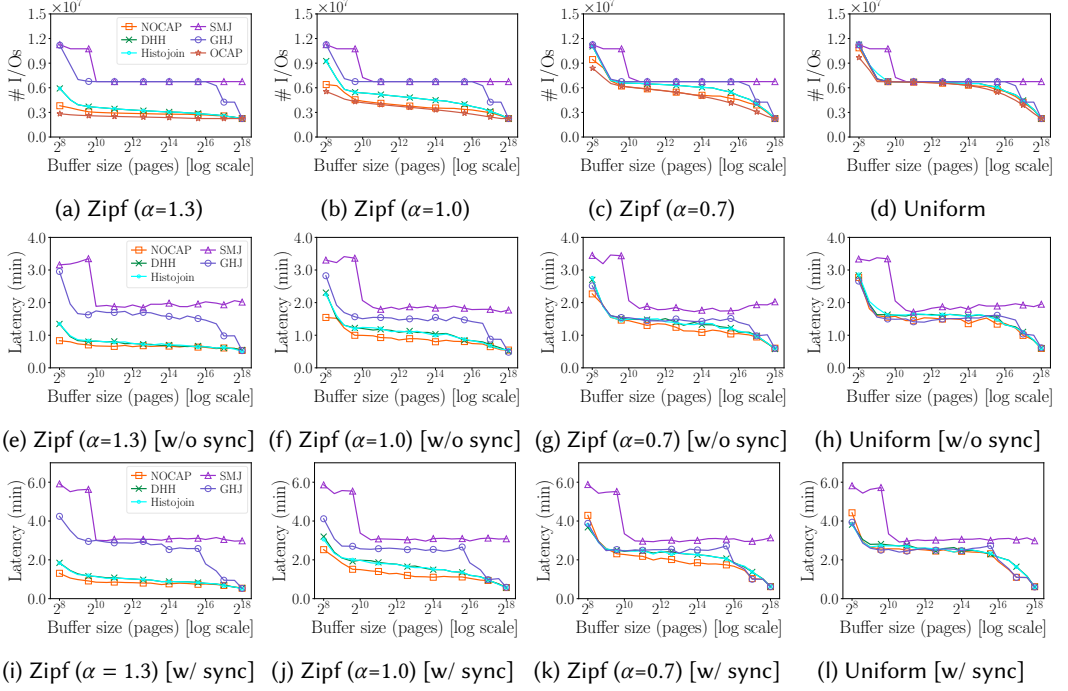
Fig. 8. While state-of-the-art skew optimization in DHH helps reduce the I/O cost, NOCAP can better exploit the correlation skew to achieve even lower I/O cost and latency. The benefit of NOCAP is more pronounced with skew correlation.
