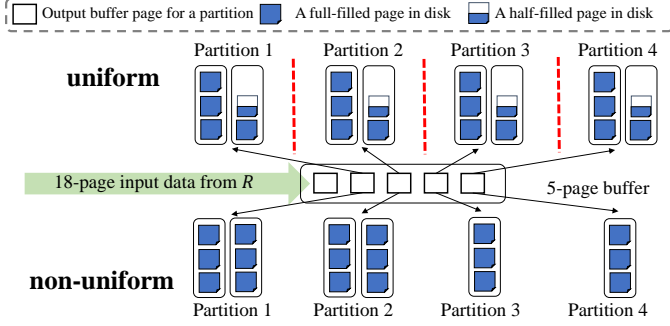
Fig. 7. An illustration of the uniform and non-uniform partitioning on the inner relation R , with a 5-page buffer (with 4 pages for partitioning R and 1 page for streaming the input). In NBJ, the maximum #chunks loaded at a time is 3-page long (with 1 page for streaming S and 1 page for the output assuming F = 1.0 ). Uniform partitioning leads to 4 partitions with each having 18/4 = 4.5 pages worth of data. One needs to read S twice for each partition. As a comparison, rounded hashing with n/c_R = 6 and m = 4 generates 2 partitions with each having 6 pages, and 2 partitions with each having 3 page worth of data. In that way, partitions 1 and 2 need two passes on the corresponding partitions in S , while partitions 3 and 4 only need a single pass.
