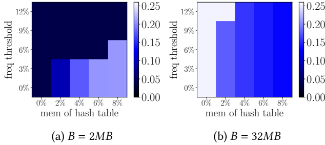
Fig. 11. DHH requires careful tuning to achieve its best performance, which is still slower than NOCAP.
