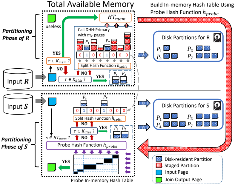
Fig. 5. An illustration of the hybrid partitioning workflow of NOCAP. Partitions P_4 and P_7 are spilled to disk when invoking DHH, while P_1 and P_2 are written to disk due to designated partitioning by f_{disk} . Other records in R either have keys from K_{mem} or stage in memory when invoking DHH, which will be inserted to the in-memory hash table HT_{mem} .
