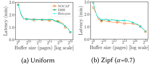
Fig. 10. With noisy MCVs, both DHH and NOCAP have similar performance to Figures 8h and 8g.
