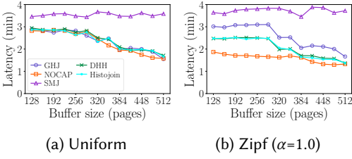
Fig. 9. When the memory is limited, NOCAP can even reach 10% speedup with uniform workload.
