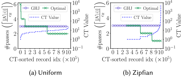
Fig. 4. A comparison of the number of passes required for the outer relation S between the partitioning adopted by DHH/GHJ and our optimal partitioning, assuming B \leq \sqrt{\|R\|} \cdot F (DHH without skew optimization downgrades to GHJ), n_R = 1M , n_S = 8M , F = 1.02 and B = 320 pages. Moreover, the record size of R is 1KB , thus R occupies 250K pages. In (a), random (uniform) partitioning (GHJ), the partition size is around 250K/319 \approx 784 pages which require \lceil 783/(318 \times F) \rceil = 3 passes to scan every partition of S . In contrast, the optimal partitioning allows the number of passes to vary from 2 to 6, which follows a non-monotonically decreasing trend as CT value increases. When we have a skewed correlation (b), a similar pattern is observed. Further, the optimal partitioning naturally excludes records with CT[i] = 0 .
