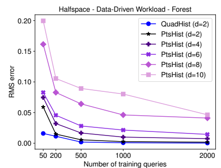
Figure 20: RMS error vs. training size on halfspace queries.
