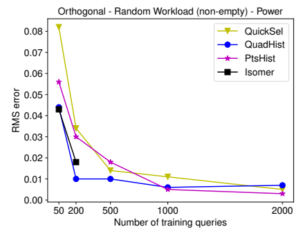
Figure 14: RMS Error vs. training size on non-empty queries in random workload of Power.
