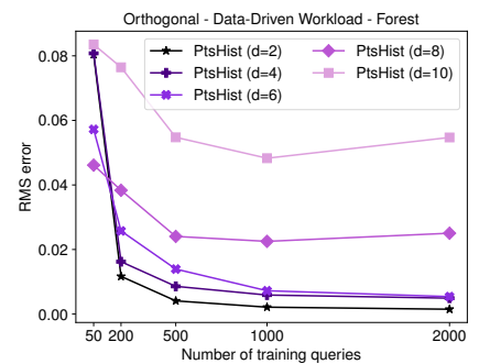
Figure 17: RMS error vs. training size on orthogonal ranges.
