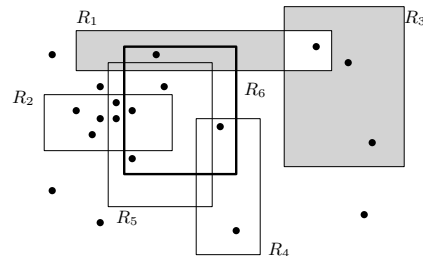
Figure 1: An illustration of the learned selectivity problem. There are 20 points in the dataset D and 5 training queries R_1, R_2, R_3, R_4, R_5 with their selectivities given by s_D(R_1) = 0.1 , s_D(R_2) = 0.3 , s_D(R_3) = 0.15 , s_D(R_4) = 0.1 and s_D(R_5) = 0.25 . The goal is to estimate the selectivity of an unknown query R_6 (in bold), and the correct answer in this example is 0.25. The shaded area will be explained in Section 2.3.
