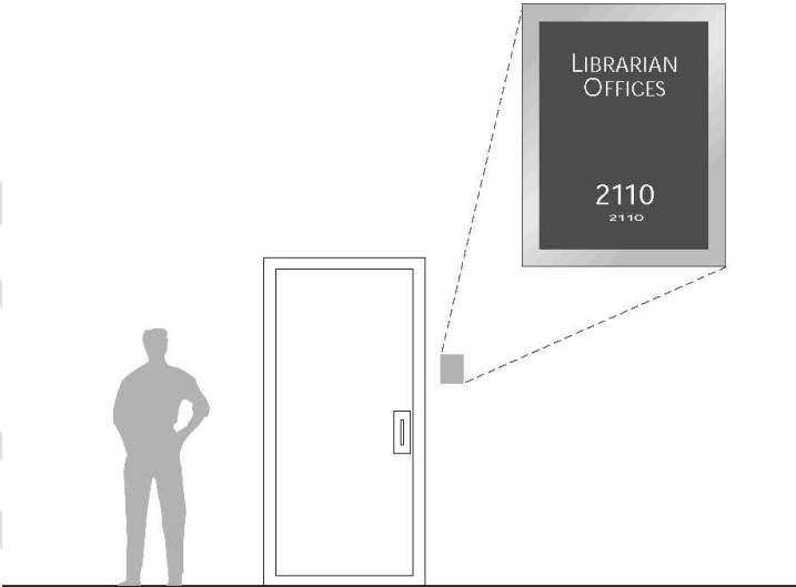
SIGN TYPE A3/00 - Large Door ID Sign
