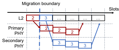
Figure 7: Visualization of pipelined slot processing in Orion.
