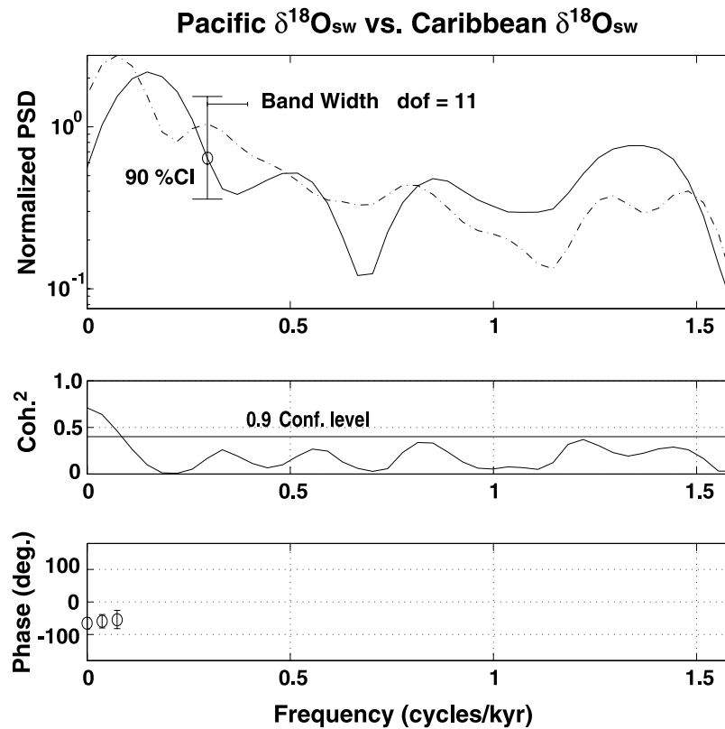
Figure 6. Cross-spectral, coherency, and phase calculations based on a Schultz fast Fourier transform that allows for nonconstant delta-T [Schulz and Stategger, 1997; Schulz and Mudelsee, 2002] comparing EPWP \delta^{18}\text{O}_{\text{sw}} (solid line) with Caribbean \delta^{18}\text{O}_{\text{sw}} (dashed line) [Schmidt et al., 2004]. Phases are only calculated for \text{Coh}^2 values that exceed the 90% confidence level. Positive (negative) phases indicate a lead (lag) of the EPWP \delta^{18}\text{O}_{\text{sw}} relative to Caribbean \delta^{18}\text{O}_{\text{sw}} . Bandwidths and 90% confidence levels are indicated.
