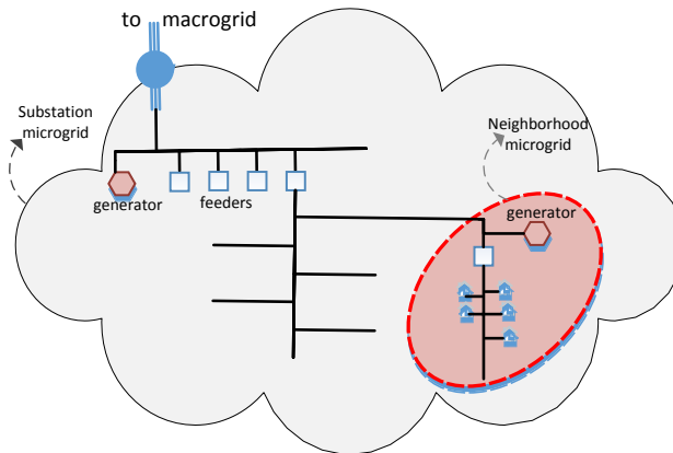
Fig. 15.9 A microgrid model
