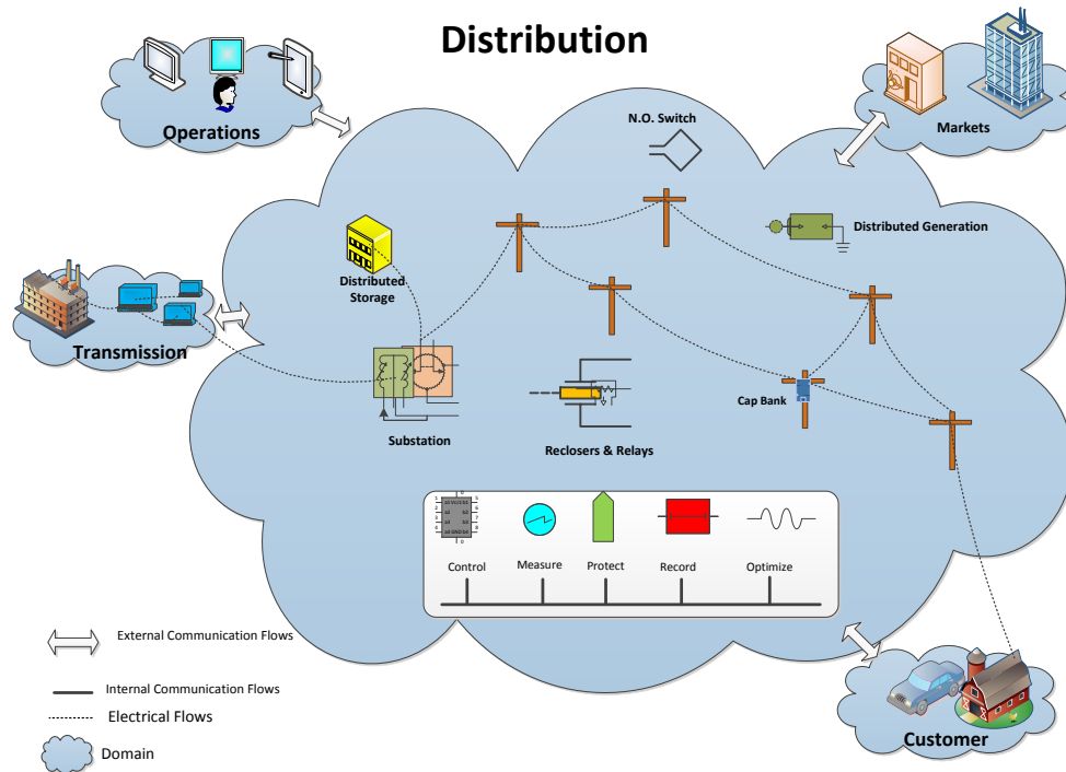
Fig. 15.4 Distribution Domain of NIST's Smart Grid Conceptual Model
