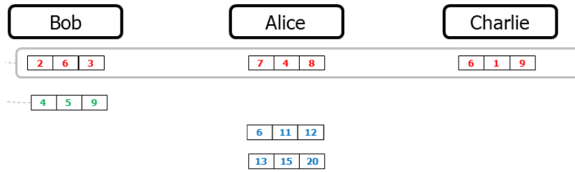
Fig. 15.19 Alice receives Bob's transmission
