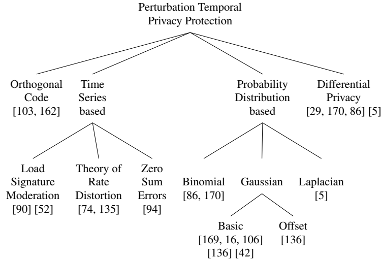
Fig. 15.24 Perturbation-based temporal privacy-provisioning techniques for the Smart Grid
