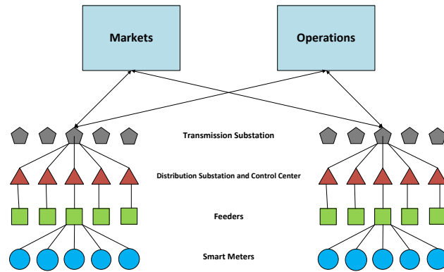
Fig. 15.8 SG communications architecture
