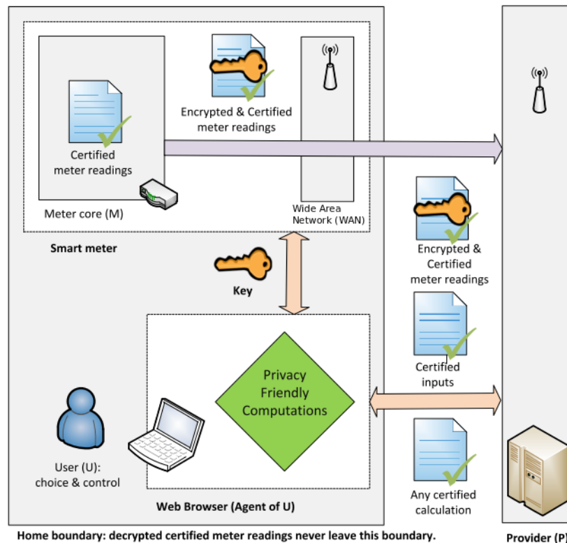
Fig. 15.22 Interaction among various parties involved in a smart metering scenario [137].
