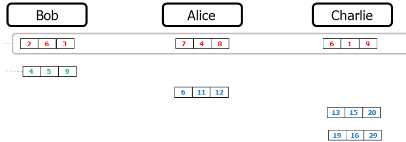
Fig. 15.20 Charlie receives Alice's transmission
