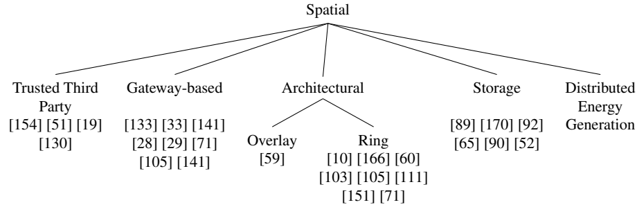
Fig. 15.14 Spatial privacy-provisioning techniques for the Smart Grid
