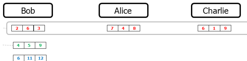
Fig. 15.18 Bob's secret random values added to his own secret
