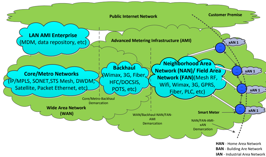
Fig. 15.5 Smart Grid Advanced Metering Infrastructure reference architecture
