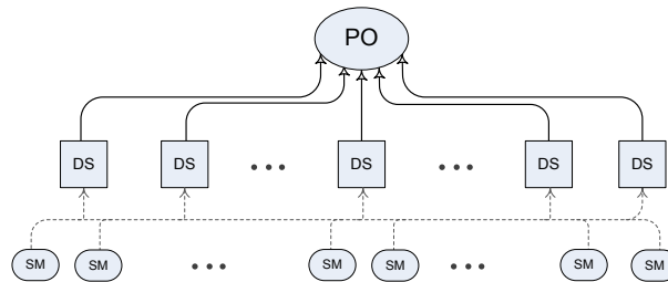
Fig. 15.23 A three-layer Smart Grid architecture. PO: power operator, DS: distribution substation, SM: smart meter
