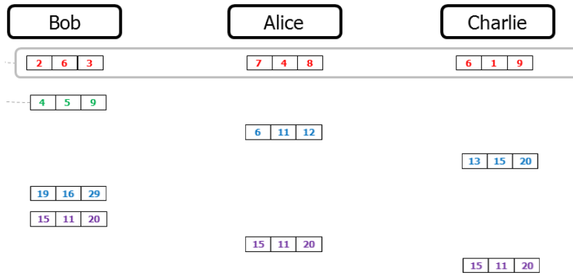
Fig. 15.21 Bob receives Charlie's transmission and computes the sum
