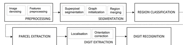
Figure 1: Overview of the system
