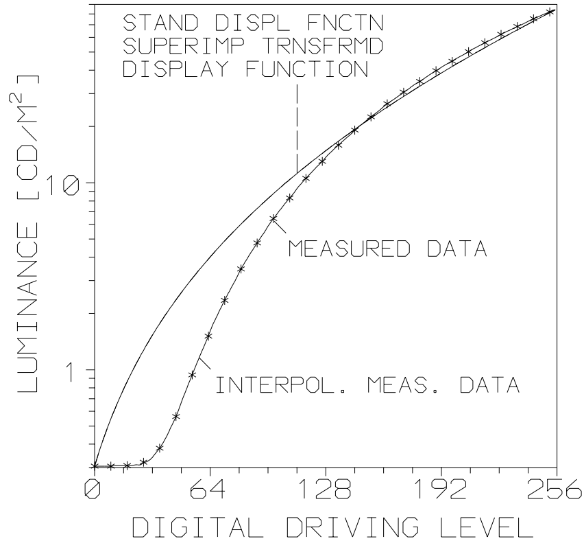
Figure D.1-3. Measured and interpolated Characteristic Curve, Grayscale Standard Display Function and transformed Display Function of an emissive Display System. The transformed Display Function for this Display System matches the Grayscale Standard Display Function and the two curves are superimposed and indistinguishable.
