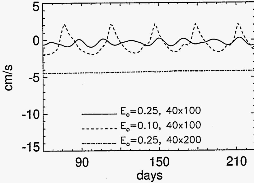
Figure 6. The difference between the elastic velocity in the center of the domain and the corresponding steady state value of the viscous-plastic velocity. The magnitude of E controls the frequency and amplitude of the oscillation, a two-dimensional effect that disappears when the grid is extended in the transverse direction. On the larger domain, the 2D elastic solution agrees well with the 1D solution, about 4 \text{ cm/s} below the steady state viscous-plastic value.
