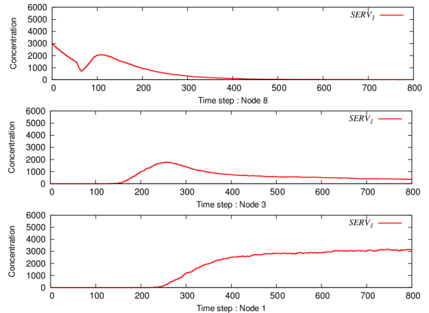
Fig. 9. Scenario 2: Concentration changes of SERV on nodes 8 (top), 3 (middle), and 1 (bottom)
