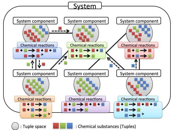
Fig. 2. Overview of chemical-inspired tuple space model
