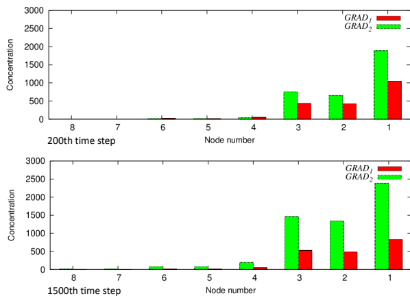
Fig. 8. Scenario 1: Gradient field for services at 200 th time step (top) and 1,500 th time step (bottom)
