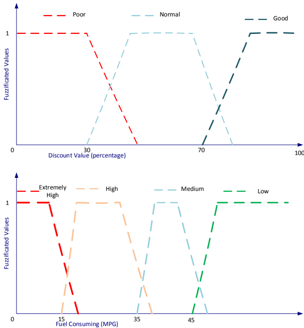
Fig. 8. Membership functions for Discount and Fuel Consuming
