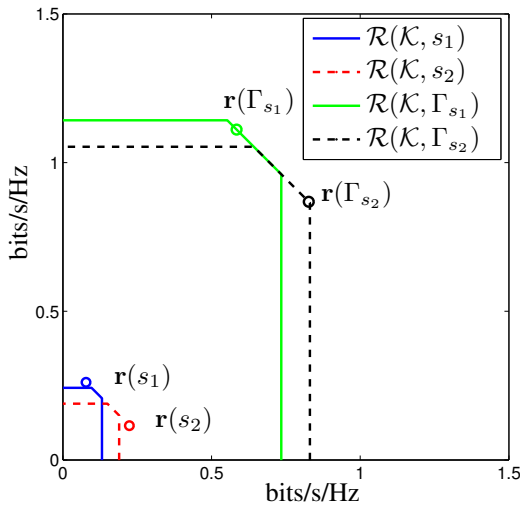
Fig. 1. Example 3.1. \mathbf{r}(\Gamma_s) \in \mathcal{M}(\mathcal{K}, \Gamma_s) , for s = s_1, s_2 , but \mathbf{r}(s) \notin \mathcal{R}(\mathcal{K}, s) , for s = s_1, s_2 , where [\mathbf{r}(s)]_{s \in \mathcal{S}} = \Phi^{-1}[\mathbf{r}(\Gamma_s)]_{s \in \mathcal{S}} .
