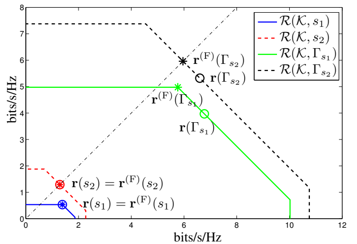
Fig. 2. Example of situation in (7) with two users and two states, in which the state-wise allocations are fair in the respective channel states but the relative long-run allocations are not fair in the respective long-run processes. The allocations indicated with the asterisk are fair, while the circle describes the actual computed allocations.
