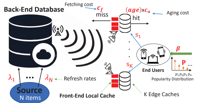
Fig. 1: Setting of Fresh Caching for Dynamic Content
