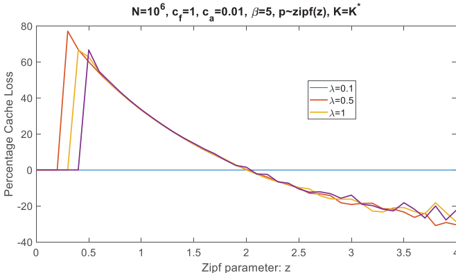
Fig. 4: Percentage cache loss of the optimal caching policy cache occupancy as our performance metric. Such a metric is defined as:
