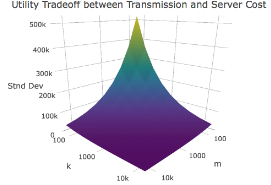
(b) Fixing \epsilon = 2 and data distribution with n = 100,000,000
