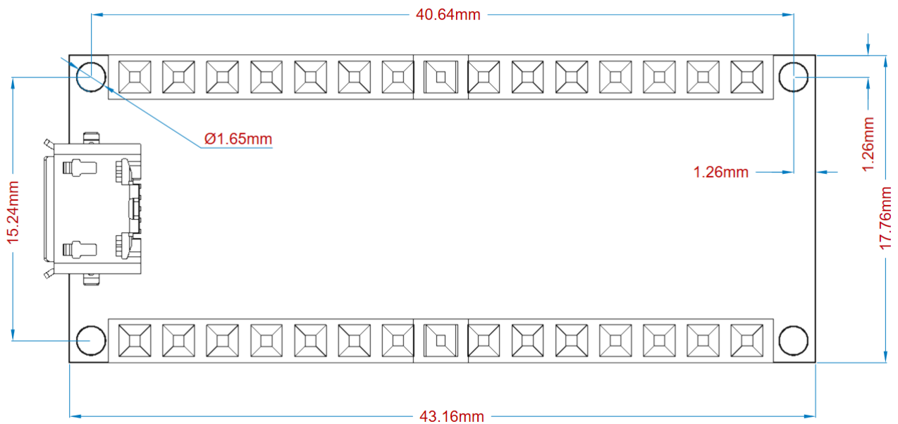
Board layout
