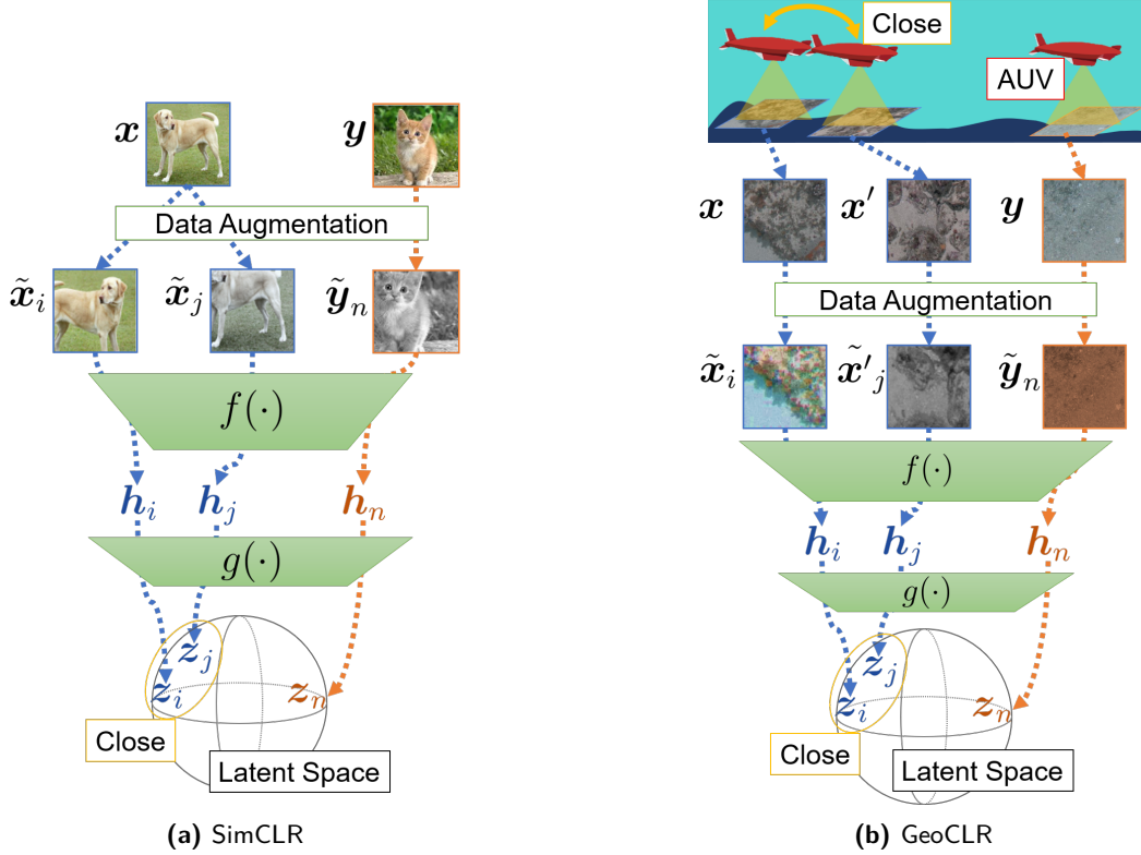
Figure 1. Overview of SimCLR and the proposed GeoCLR. The two methods apply different conditions to generate similar pairs of images to implement contrastive learning. (a) In SimCLR, similar image pairs [\tilde{x}_i, \tilde{x}_j] are generated by applying different random augmentations to the same image x . (b) The proposed GeoCLR generates similar pairs [\tilde{x}_i, \tilde{x}'_j] using different images that were taken from physically nearby locations, x and x' . The large range of variability captured in the generated similar pairs allows for robust CNN training.
