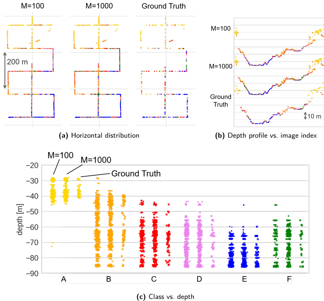
Figure 9. Class distribution of dive 08 with M = 100 annotations by F8, M = 1000 annotations by F4 in Table 3 and ground truth. The same color scheme as Figure 3 is applied.
