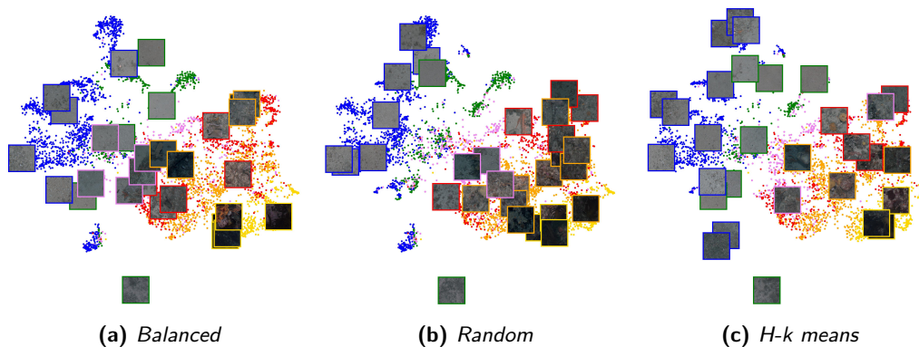
Figure 4. Comparison of training data sampling strategy. M = 30 images are selected by (a) balanced , (b) random , and (c) H-k-means strategy. The selected images are shown on t -distributed stochastic neighbor embedding ( t -SNE) visualization of latent representations obtained by GeoCLR. While random sampling fails to select from the center area, H-k-means successfully selects the images in the relatively sparse areas so that a more informative training dataset is gained. Similarly, balanced fails to sample regions of the latent space where there are more densely populated regions of the same class. In these situations, class assigned by the classifier will depend on the class of training examples that happen to be nearby. The same color scheme as Figure 3 is applied.
