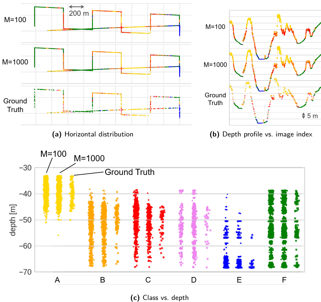
Figure 7. Class distribution of dive 01 with M = 100 annotations by F8, M = 1000 annotations by F4 in Table 3 and ground truth. The same color scheme as Figure 3 is applied.
