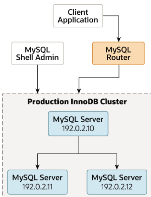
Figure 7.2 Production Deployment
