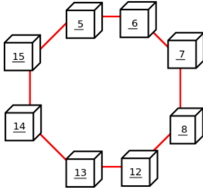
Figure 17.9 Circular Arrangement of MySQL Cluster Nodes
