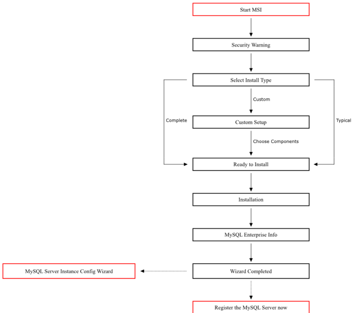
Figure 2.17 Installation Workflow for Windows Using MSI Installer
