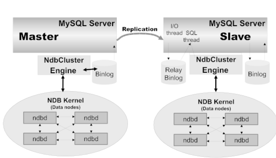
Figure 17.13 MySQL Cluster-to-Cluster Replication Layout
