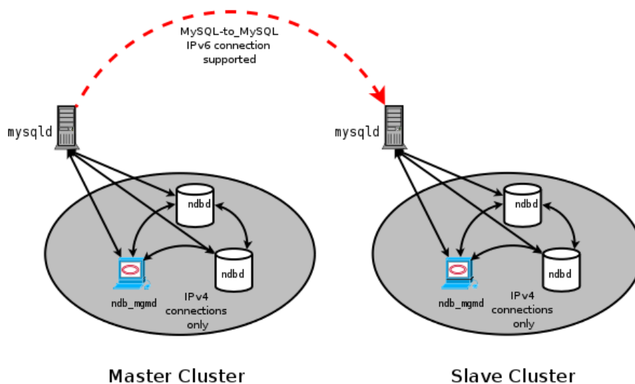
Figure 17.16 Replication Between SQL Nodes Connected Using IPv6
