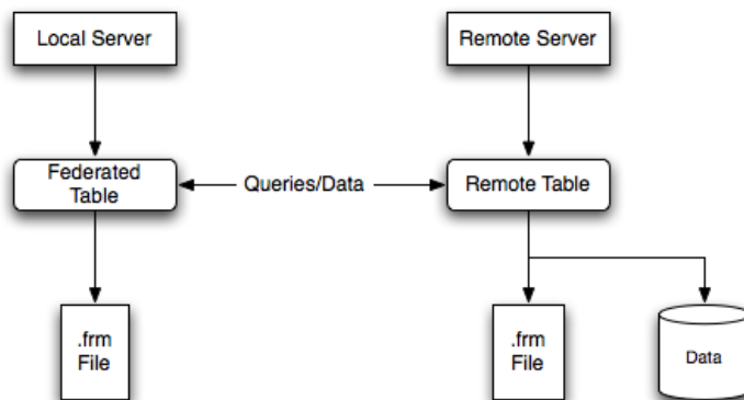
Figure 14.1 FEDERATED Table Structure
