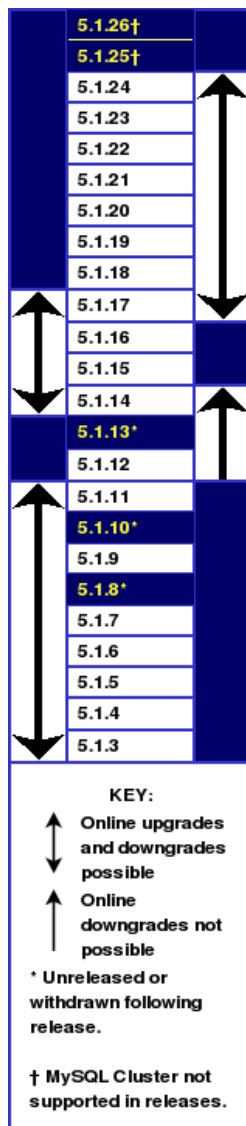
Figure 17.7 MySQL Cluster Upgrade and Downgrade compatibility, MySQL Cluster 5.1
