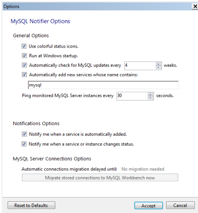
Figure 2.11 MySQL Notifier Options menu
