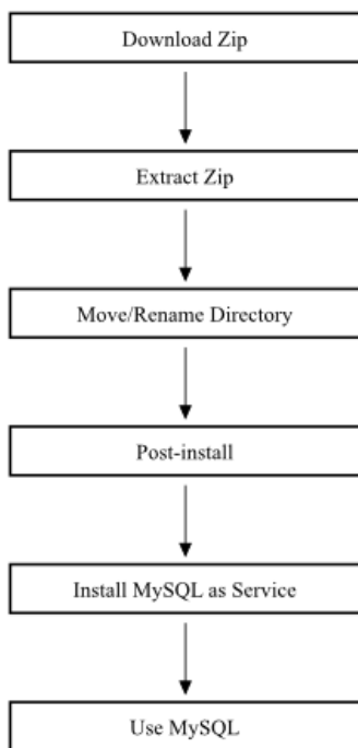
Figure 2.8 Installation Workflow for Windows Using Zip
