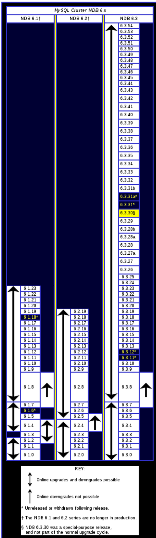
Figure 17.6 MySQL Cluster Upgrade and Downgrade compatibility, MySQL Cluster NDB 6.x
