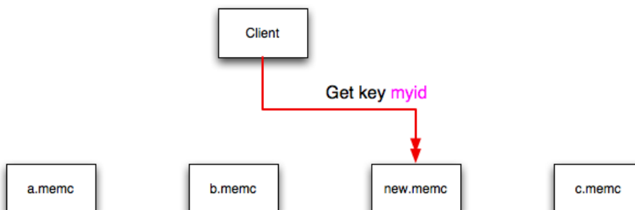
Figure 15.4 memcached Hash Selection with New memcached instance
