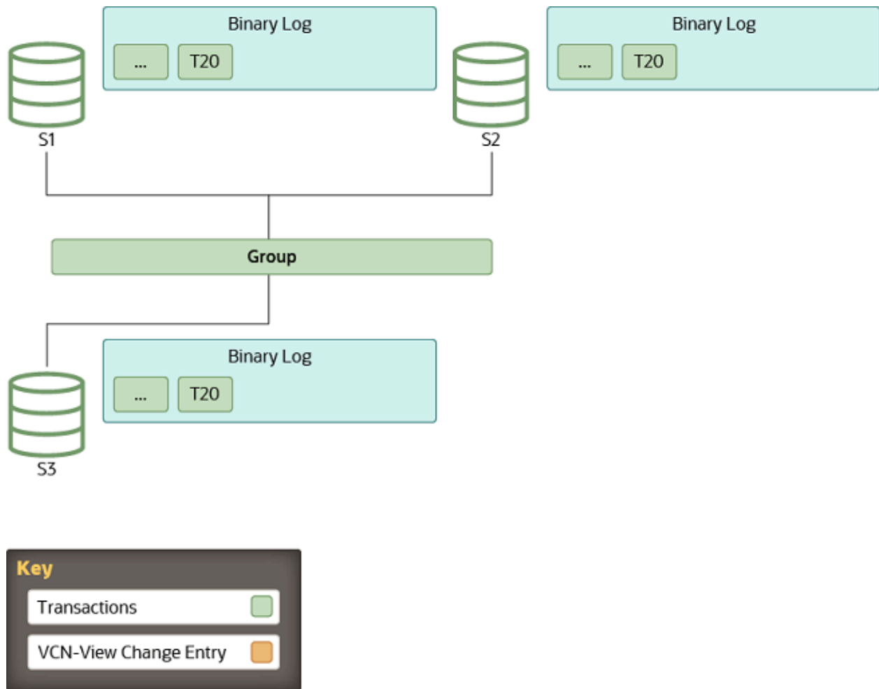
Figure 18.8 Stable Group
