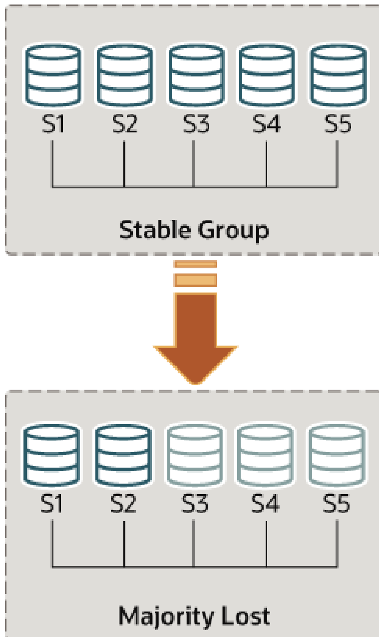
Figure 18.14 Losing Quorum
