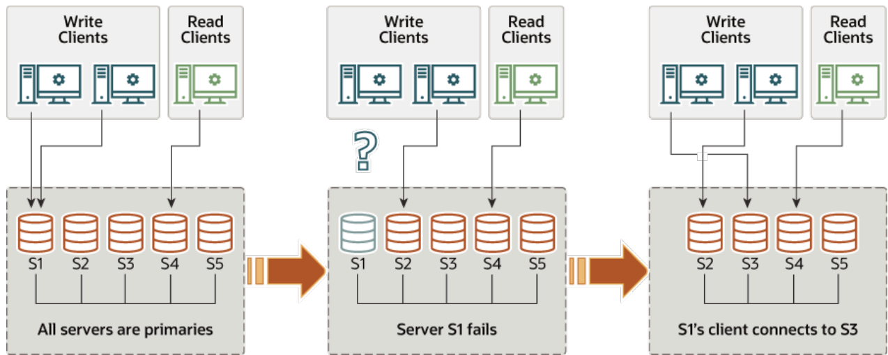
Figure 18.5 Client Failover
