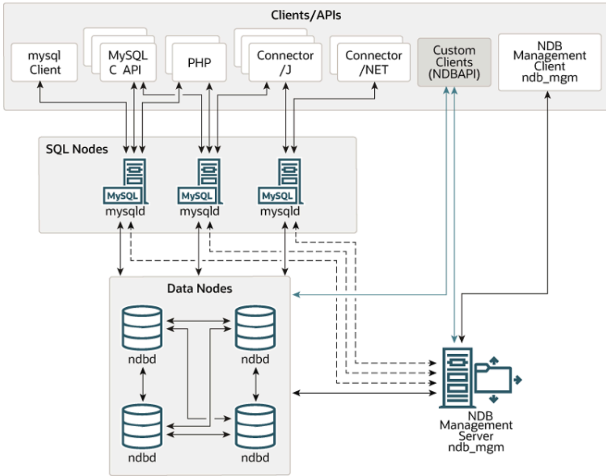
Figure 23.1 NDB Cluster Components
