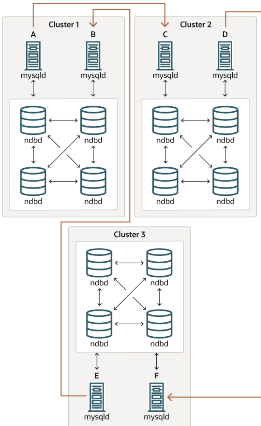
Figure 23.15 NDB Cluster Circular Replication Where Not All Sources Are Replicas
