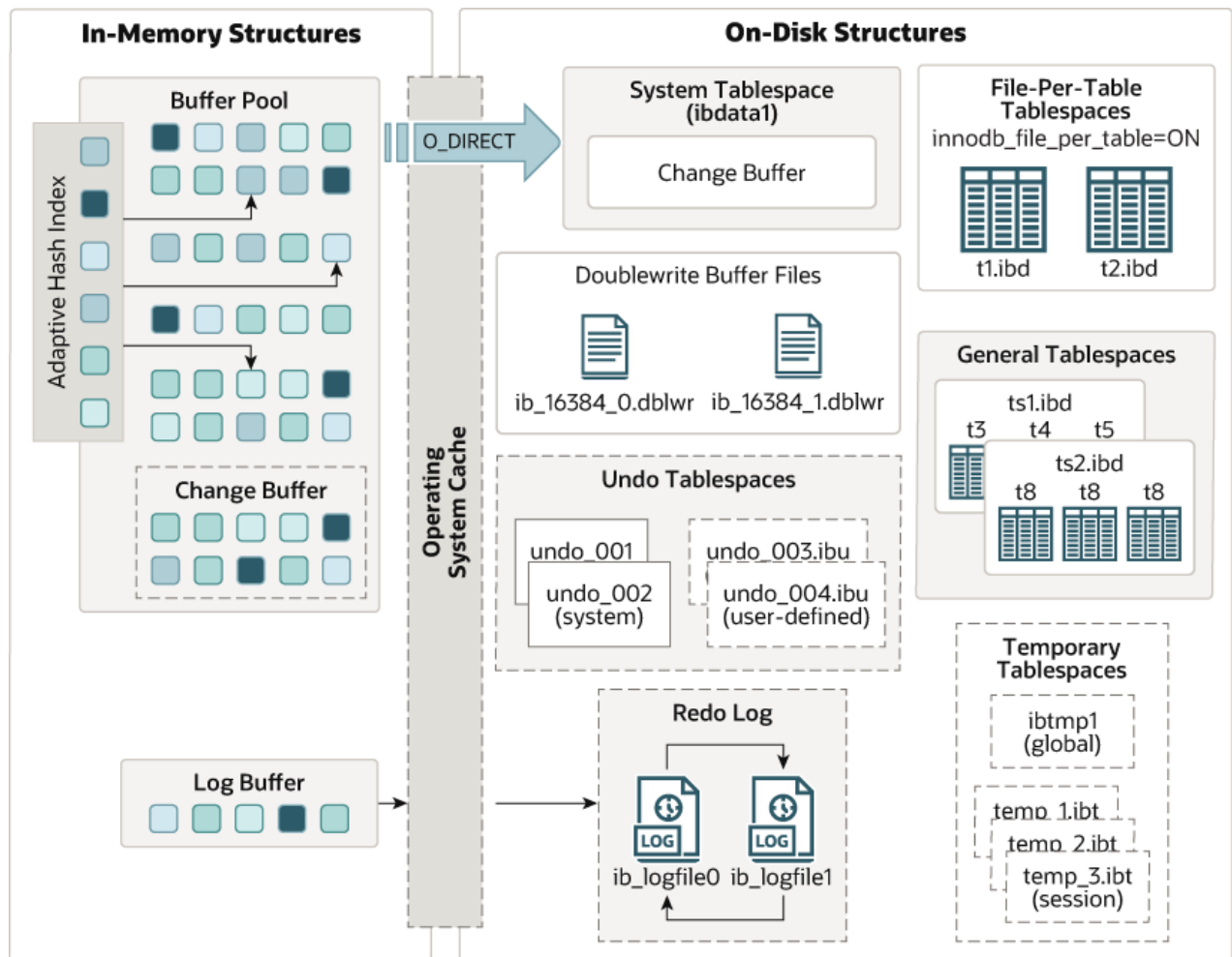
Figure 15.1 InnoDB Architecture
