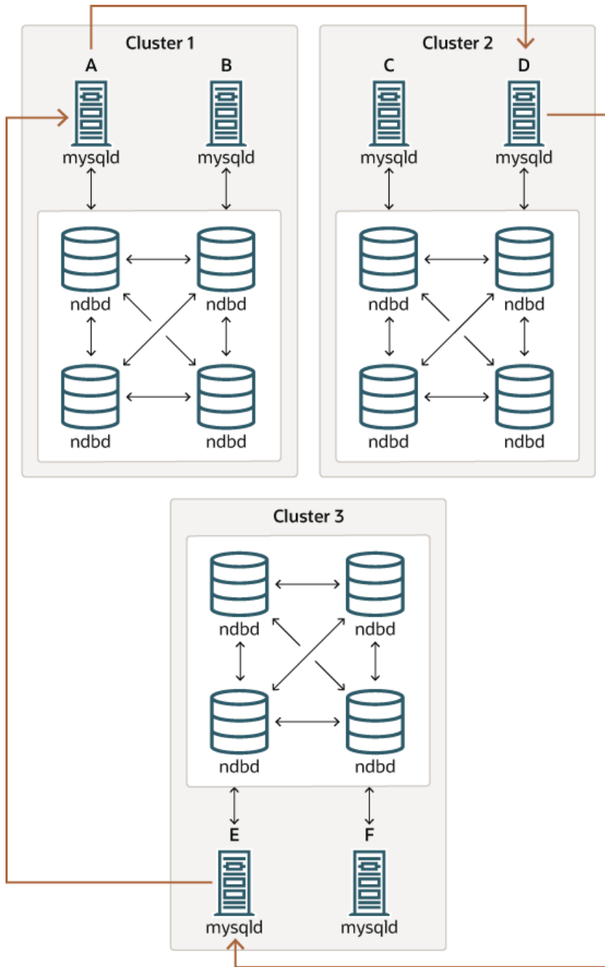
Figure 23.14 NDB Cluster Circular Replication with All Sources As Replicas
