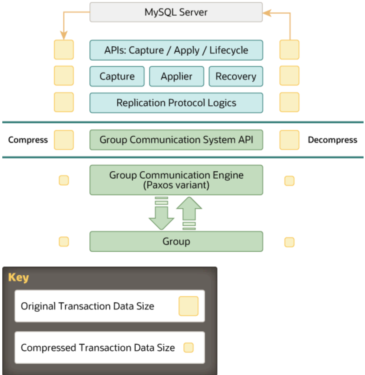
Figure 18.13 Compression Support
