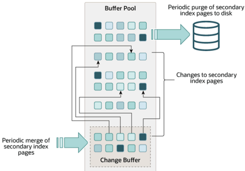
Figure 15.3 Change Buffer
