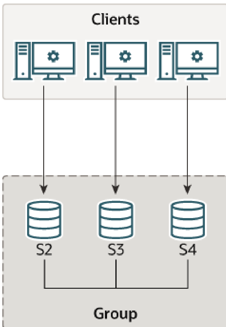
Figure 18.7 Group Architecture
