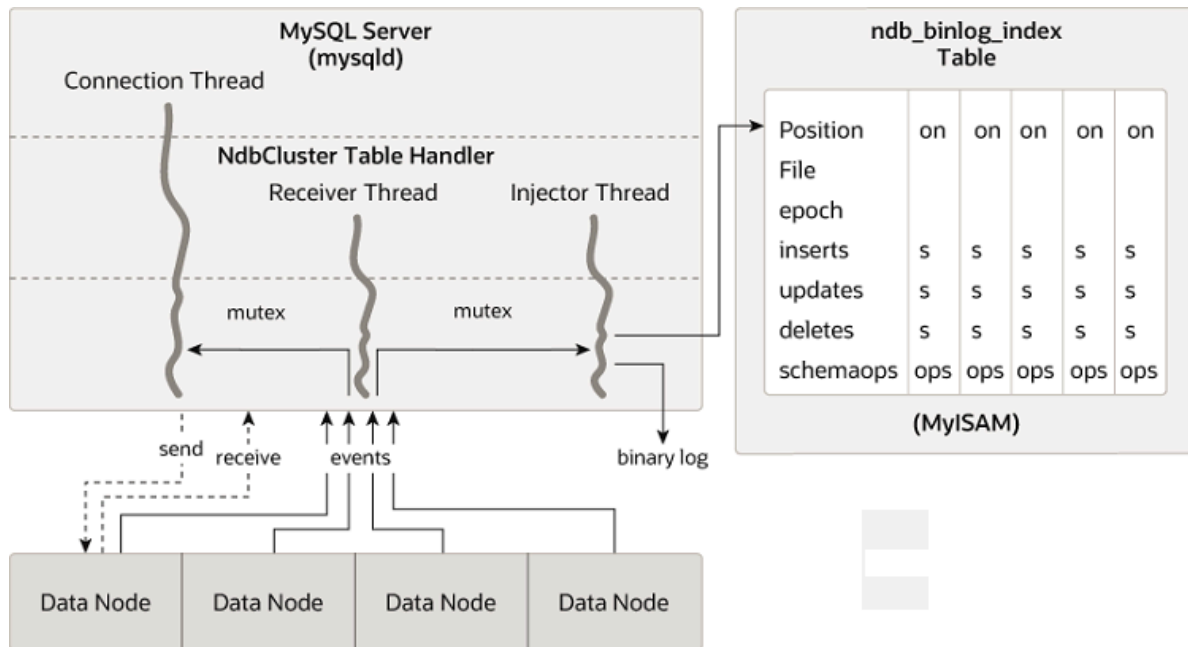
Figure 23.13 The Replication Source Cluster
