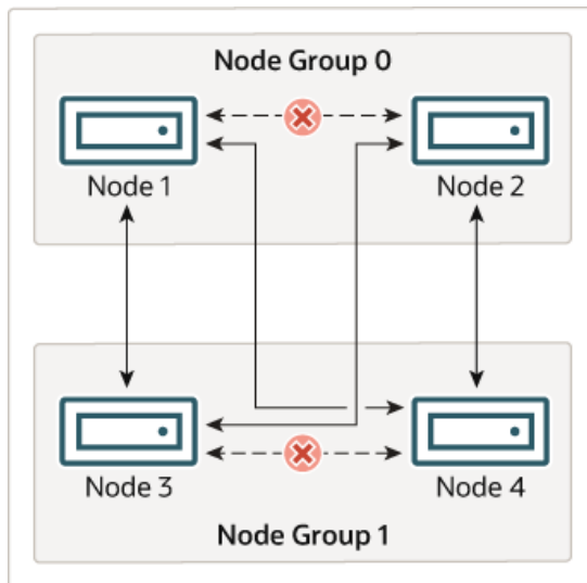
Figure 23.3 Nodes Required for a 2x2 NDB Cluster
