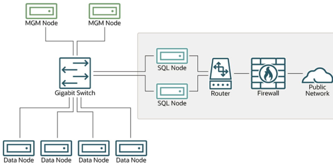
Figure 23.7 NDB Cluster with Hardware Firewall
