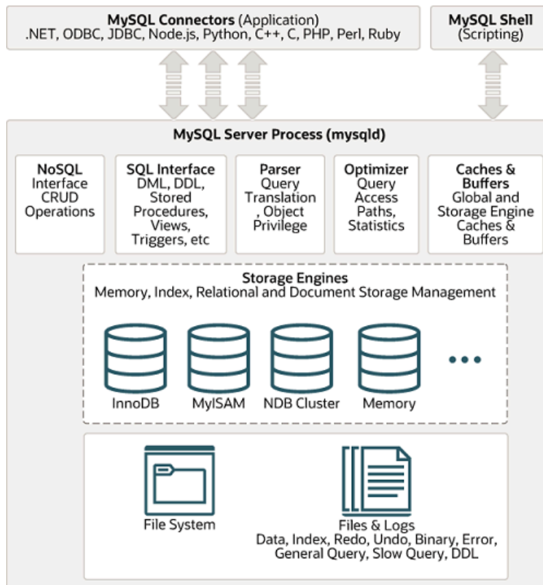
Figure 16.3 MySQL Architecture with Pluggable Storage Engines
