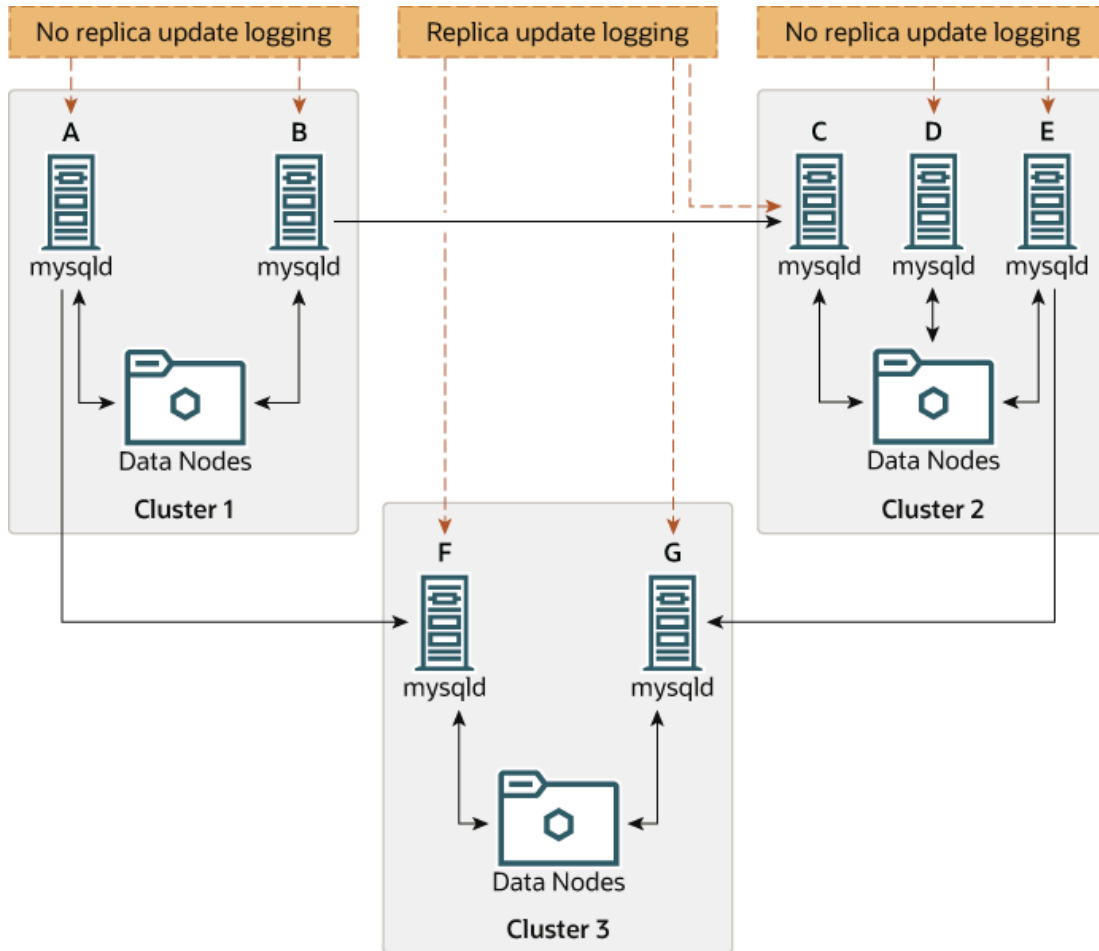
Figure 23.17 NDB Cluster Multi-Source Replication, With MySQL Servers
