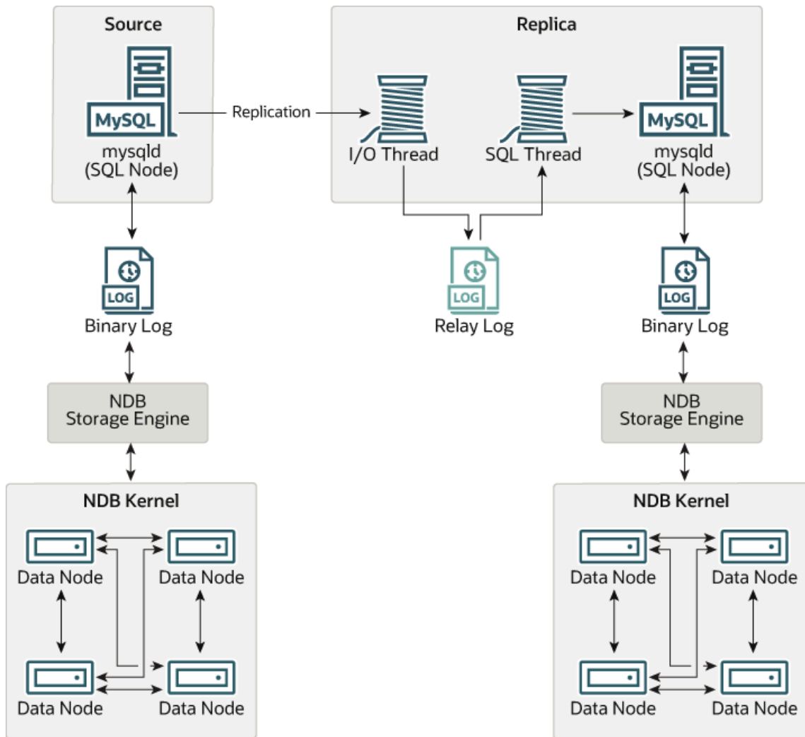
Figure 23.10 NDB Cluster-to-Cluster Replication Layout
