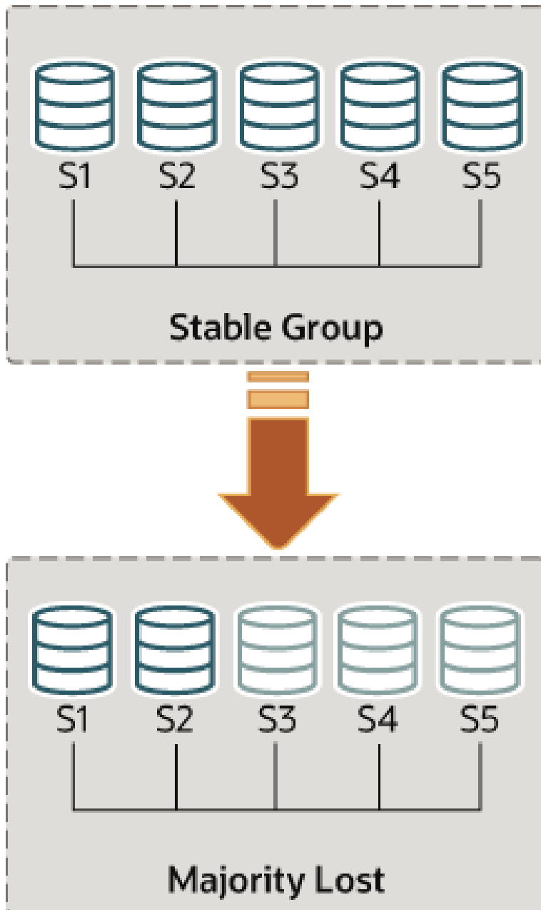
Figure 20.14 Losing Quorum
