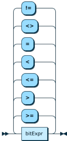
Figure 12.27 compExpr
