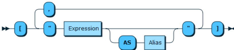
Figure 11.27 ProjectedSearchExprStrList
