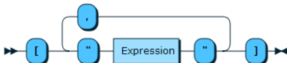
Figure 11.25 SearchExprStrList
