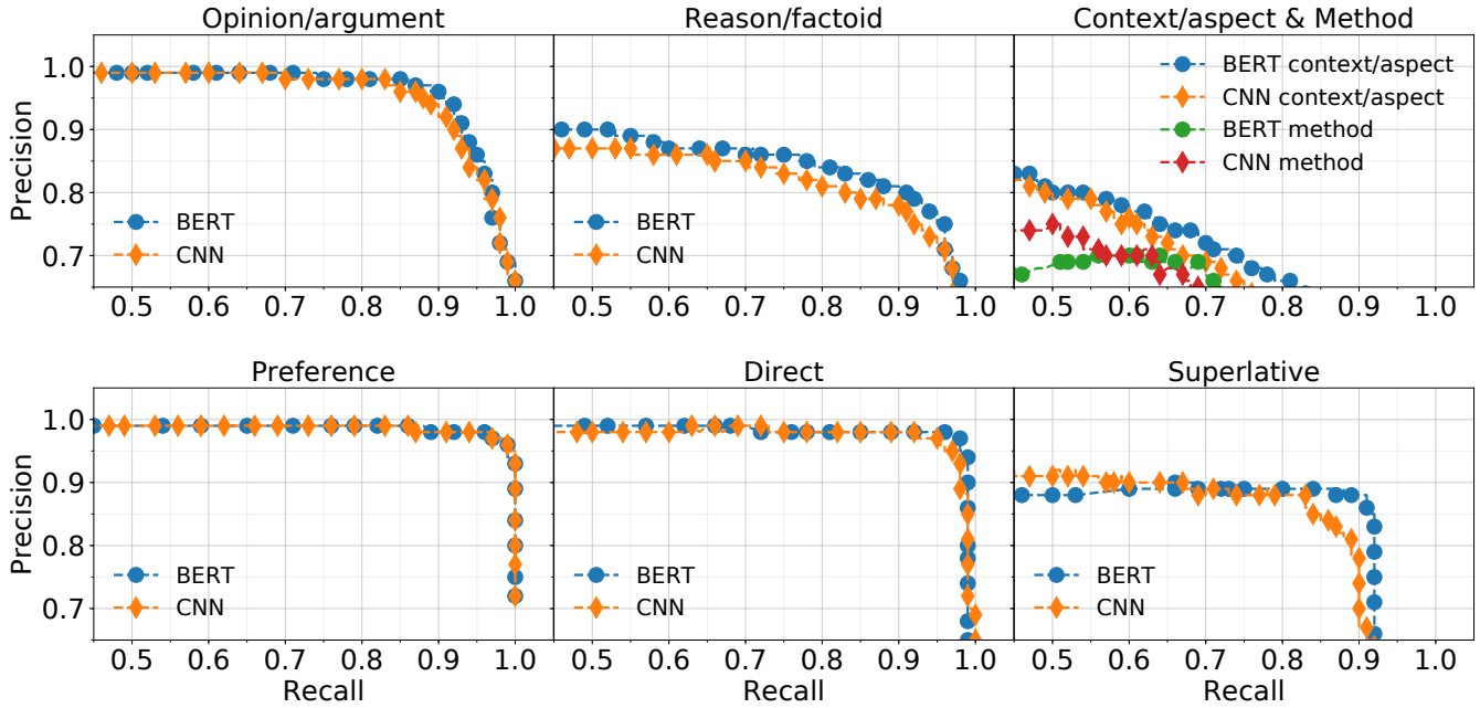
Figure 2: Precision-recall curves for the comparative subclasses on the training set (5,000 questions, ten-fold cross-validation).
